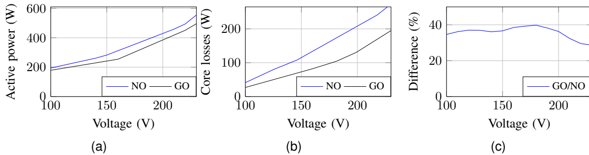
Fig. 4. (a) Active power consumption at different voltage levels. (b) Core losses at different voltage levels. (c) Difference of Core losses at different voltage levels;
