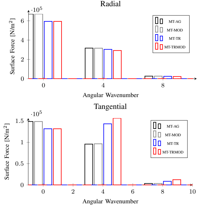
Fig. 2. Comparison of several methods for surface force density: MT-TR is the reference method at the tooth tip, and MT-TRMOD the reference at the yoke level.
