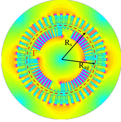
Fig. 1. Turbo-alternator: Z_s = 48 , R_{ag} = 0.8 [m] and R_s = 0.85 [m]
