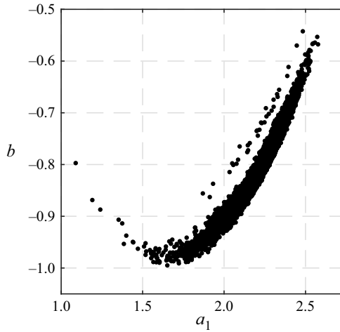
Figure 20. Actuation command b vs a_1 for the case: K^1 controlling the mode-switching regime.
