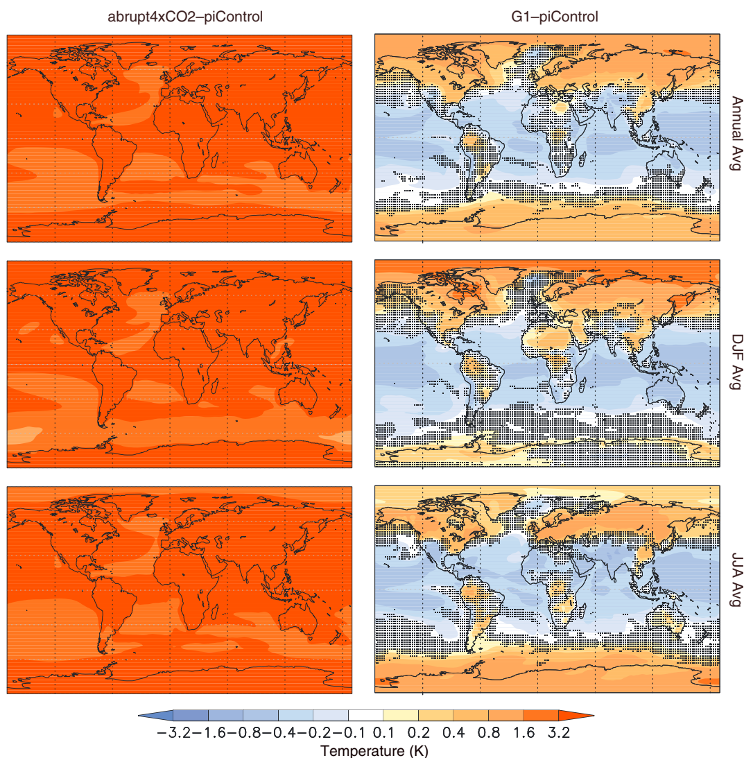
Figure 2. All-model ensemble annual average surface air temperature differences (K) for abrupt4xCO 2 -piControl (left column) and G1-piControl (right column), averaged over years 11–50 of the simulation. Top row shows annual average, middle row shows December–January–February (DJF) average, and bottom row shows June–July–August (JJA) average. Stippling indicates where fewer than 75% of the models (for this variable, 9 out of 12) agree on the sign of the difference.
