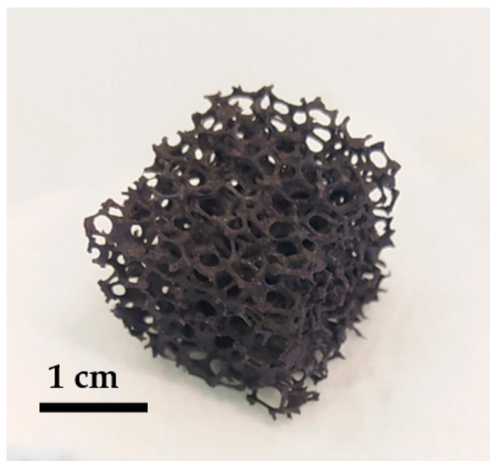
Figure 1. Picture of a pristine \text{NiFe}_2\text{O}_4 foam calcined at 1400\text{ }^\circ\text{C} .
