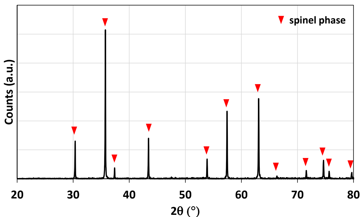
Figure 2. X-ray diffraction pattern of the \text{NiFe}_2\text{O}_4 foam after calcination at 1400\text{ }^\circ\text{C} .
