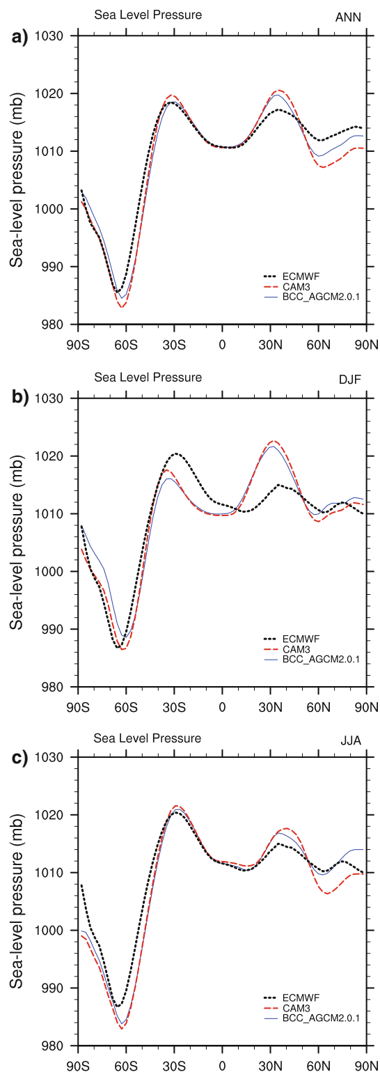
Fig. 13 The annual, DJF and JJA averaged zonal-mean SLP for the BCC_AGCM2.0.1, CAM3, and the ERA-40 reanalyses. Unit: mb
