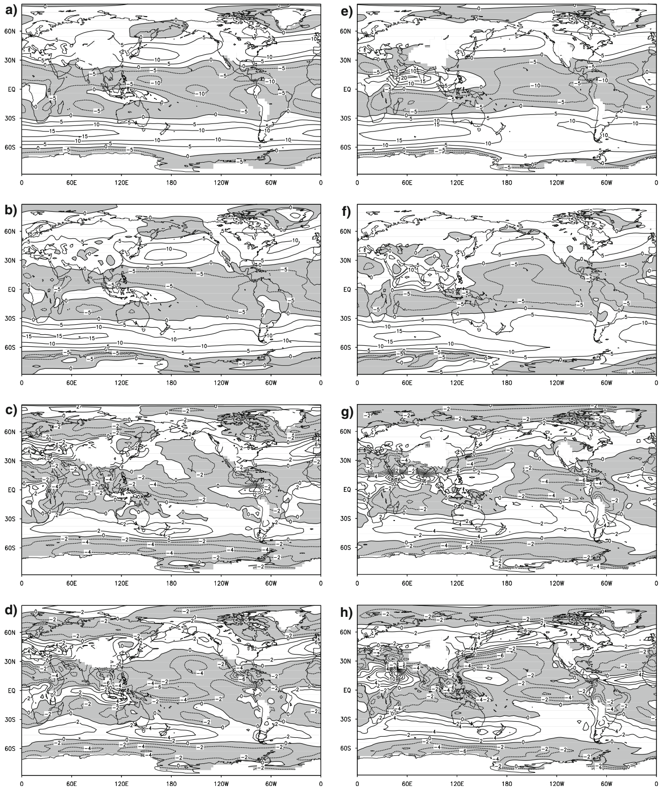
Fig. 16 The same as that in Fig. 11, but for 850-hPa zonal wind. Unit: \text{m s}^{-1} . Intervals are 5 \text{ m s}^{-1} in a , b , e , and f and 2 \text{ m s}^{-1} in c , d , g , and h
