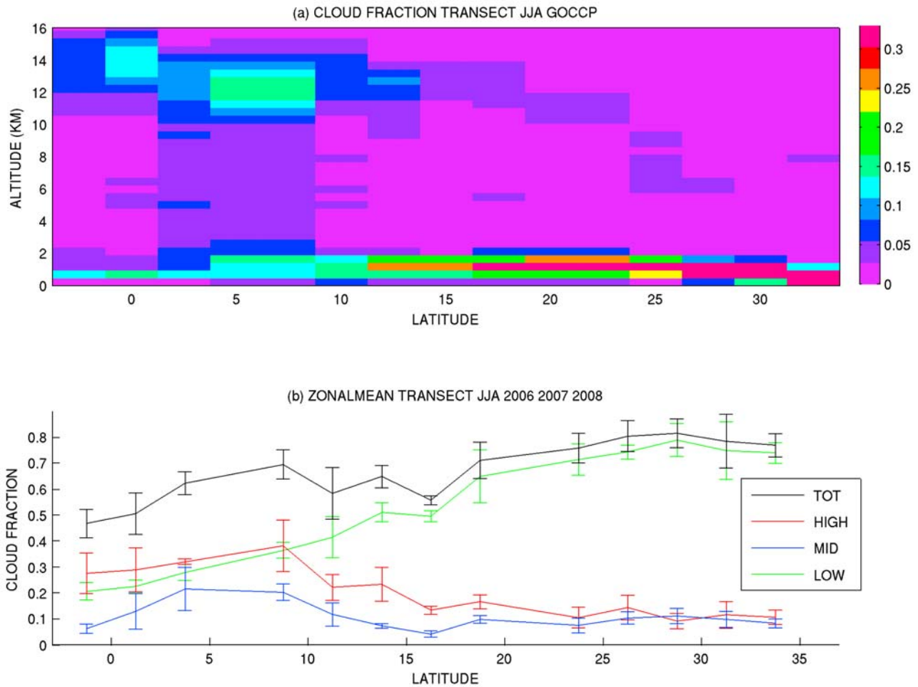
Figure 9. Cloud fraction along the GPCI Pacific Cross-Section Intercomparison (GPCI) transect (that extends over the Pacific from California to the ITCZ) in JJA: (a) vertical distribution of the cloud fraction and (b) low, middle, high, and total cloud fractions.
