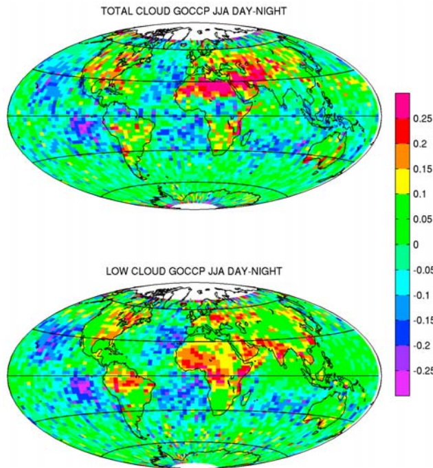
Figure 8. Cloud cover difference between daytime and nighttime GOCCP data for JJA.
