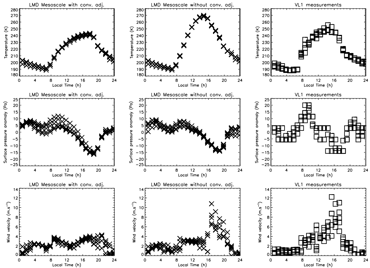
Figure 3. Comparison of the meteorological fields predicted by the mesoscale model (grid point coordinates 48.09^{\circ}\text{W} , 22.24^{\circ}\text{N} ) with Viking Lander 1 measurements (coordinates 47.95^{\circ}\text{W} , 22.27^{\circ}\text{N} ). The first level of the model is \sim 0.6 m above the surface, and the second level is \sim 3.5 m. Temperature values 1.6 m above the surface (altitude of the Viking Lander 1 sensor) are obtained by linear interpolation in the vertical dimension. Wind values 1.6 m above the surface are derived from the simulated values assuming a logarithmic wind profile with surface roughness of 1 cm. Surface pressure anomalies are computed using a daily average value. Mesoscale model results with and without convective adjustment are shown.
