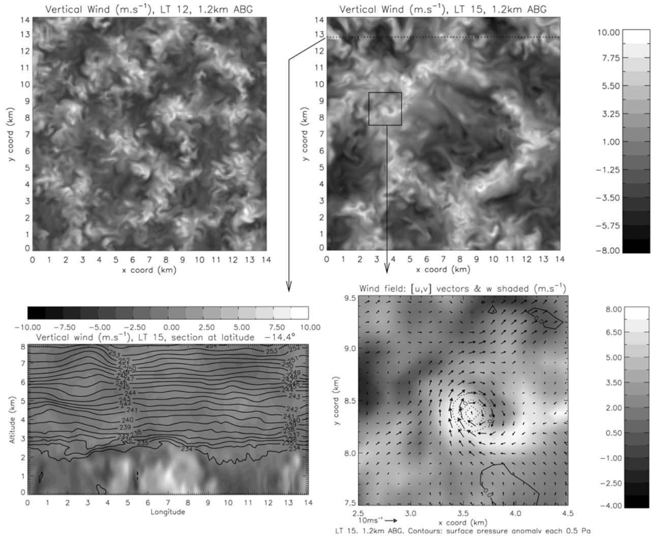
Figure 9. Instantaneous view of the simulated atmospheric circulation at microscales in Gusev Crater. (top) Vertical velocity horizontal section 1.2 km above the surface, showing the entire simulation domain. Updrafts are represented in white; downdrafts are in black. Each kilometer comprises 10 grid points, enabling a fine representation of the “large-eddy” part of the turbulence spectra, as can be observed in the images. Instantaneous fields at (left) 1200 LT and (right) 1500 LT are provided to give clues on the evolution of the polygonal structure of the convective cells. (bottom) Insights into the shaded vertical velocity field of the top right image. Note that the black and white scales are different. (bottom left) Longitude-altitude cross section of vertical velocity with potential temperature contours superimposed (1 K spacing). Note that the model top is \sim 11 km. (bottom right) Enhanced view of a particular vortical structure. Horizontal wind vectors are superimposed, as well as contours corresponding to the surface pressure perturbation (0.5 Pa spacing), obtained by subtracting from the raw surface pressure field an average surface pressure value over the whole domain. Maximal depression in the vortex core is \sim 1.5 Pa.
