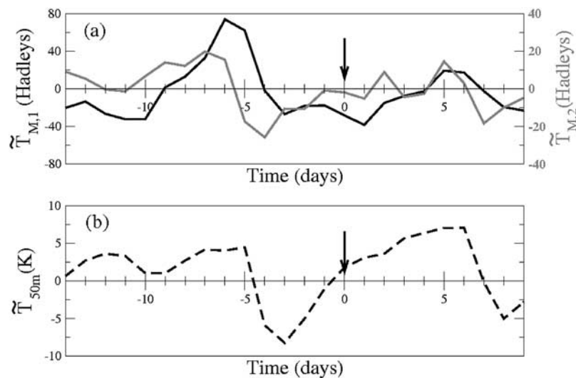
Figure 3. (a) \tilde{T}_{M,1} and \tilde{T}_{M,2} and (b) the average of \tilde{T}_{50m} over the sector [112.5^{\circ}\text{E}; 117.5^{\circ}\text{E}] \times [25^{\circ}\text{N}; 30^{\circ}\text{N}] . The time axes for Figures 3a and 3b are in days relative to 14 November 1990 (black arrow).
