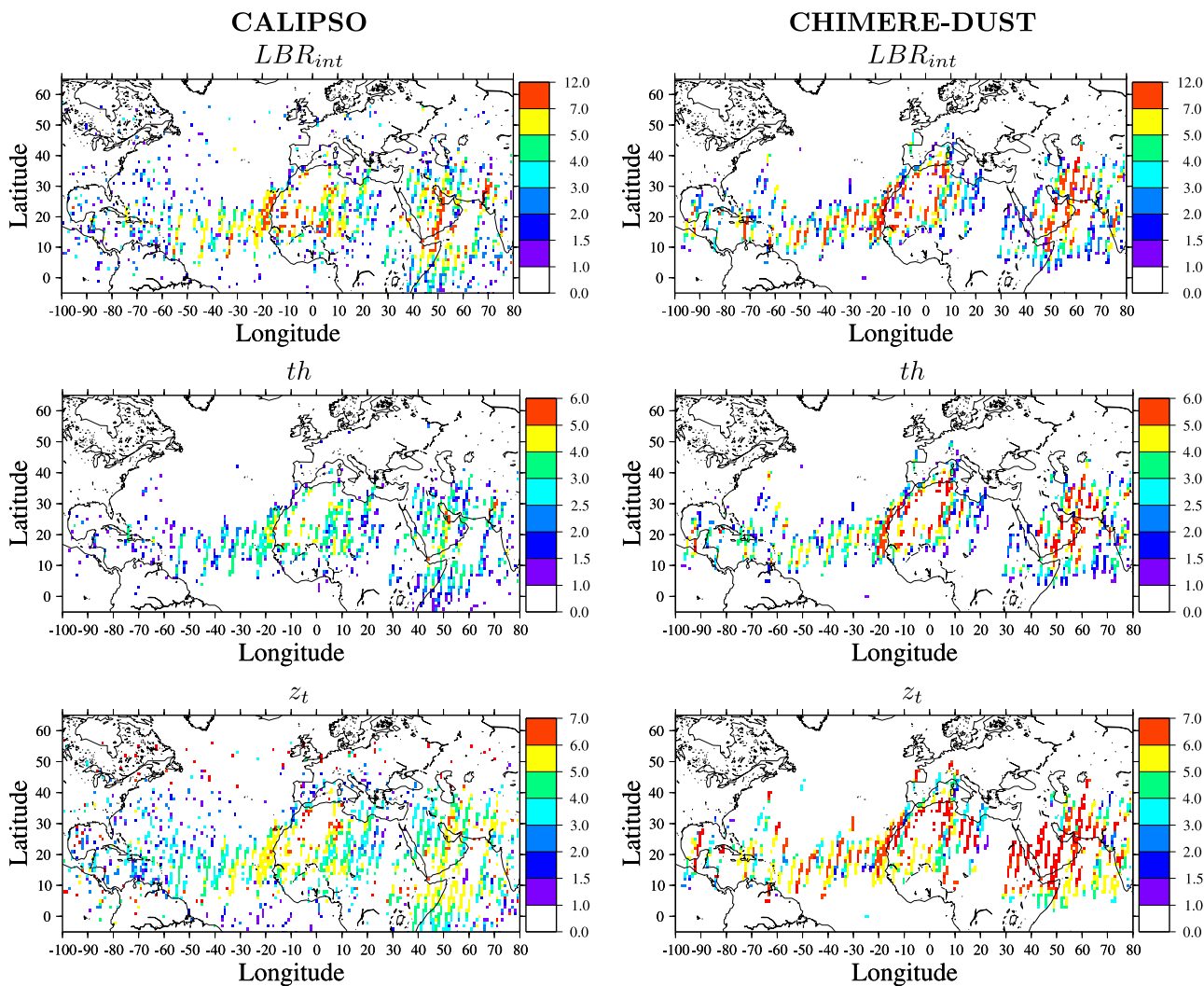
Figure 8. Maps of (top) LBR_{int} , (middle) “ th ” dust layer thickness (kilometers) and (bottom) z_t (kilometers) for the period 1 to 15 July 2006. Only nighttime data are used, and comparisons are presented for (left) the CALIPSO data and (right) the CHIMERE-DUST outputs.
