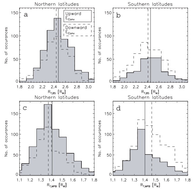
Fig. 7. Distribution of the extrapolated terminator distance of BS crossings in the (a) Northern and in the (b) Southern Hemisphere and MPB crossings in the (c) Northern and in the (d) Southern Hemisphere observed by MEX from February 2004 until November 2006. In each panel, the distributions are subdivided into whether they occur when the convective electric field is directed locally upward (solid, filled) or locally downward (dashed). The mean extrapolated terminator distances are shown for crossings that occur in the locally upward convective electric field hemisphere (solid vertical line) and in the locally downward convective electric field hemisphere (dashed vertical line).
