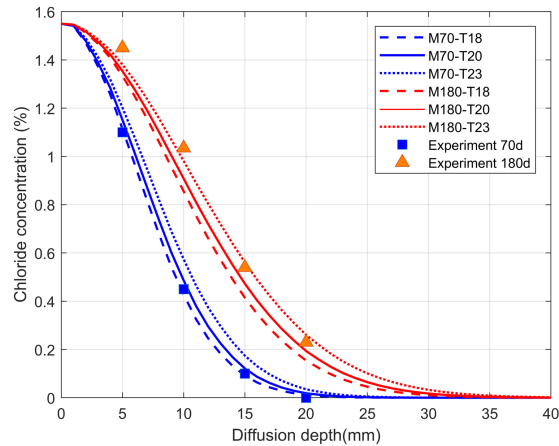
Fig. 2. Chloride diffusion model validation with data taken from [34]
