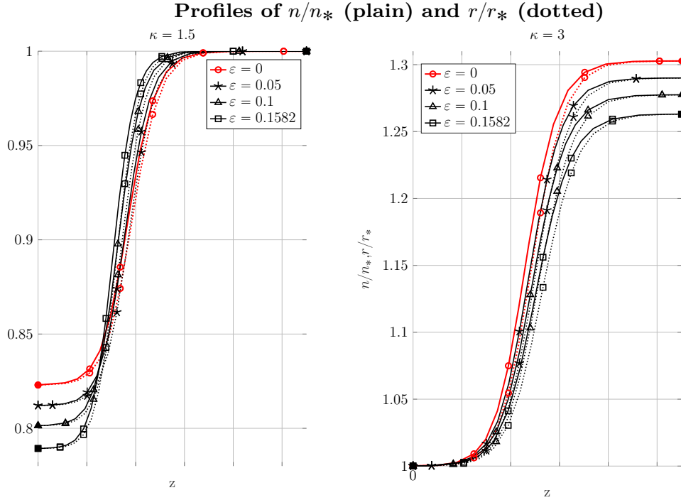
FIGURE 9. Graphs of n (plain) and r(n) (dotted) where n solves problem (5.21) for several values of \epsilon , n_* being fixed and \tau = n_*/r_* being chosen strictly less than \tau_{\#}(\kappa) (here, \tau = 0.3\tau_{\#} ). The pressure law is the \gamma -law (1.5) with exponent \gamma = 2 .
