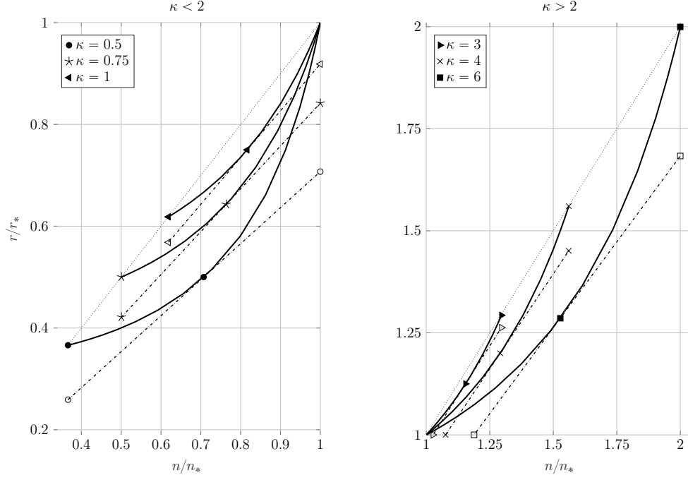
FIGURE 7. Orbits connecting (n_{\times}, r_{\kappa}(n_{\times})) to (1, 1) for several values of \kappa for the \gamma -law (1.5) with exponent \gamma = 2 . The straight line n \mapsto \tau_{\#}(\kappa)n is plotted for each value of \kappa , and the tangent point with the corresponding orbit is indicated. The markers are the same as in Figure 6.
