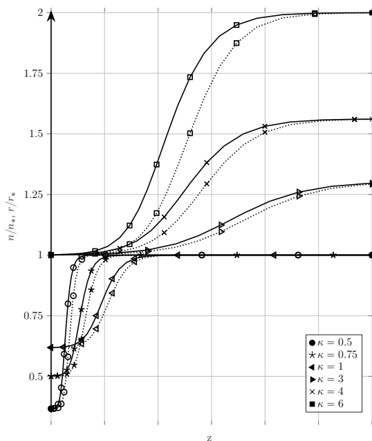
FIGURE 6. Graphs of n/n_* (plain) and r/r_* = r_\kappa(n/n_*) (dotted) where n solves problem (5.3)-(5.4) for several values of \kappa such that \tau < \tau_\# . The pressure law p is the \gamma -law (1.5) with exponent \gamma = 2 .
