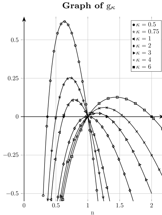
FIGURE 4. The graph of the function g_\kappa in (5.18) for the \gamma -law (1.5) with exponent \gamma = 2 . The markers are the same as in Figures 6 and 7.
