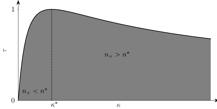
FIGURE 5. The graph of the function \tau_{\#} in the case of the \gamma -law (1.5) with \gamma = 2 . Small shocks are concentrated in a neighborhood of \kappa = \kappa_* = 2 .
