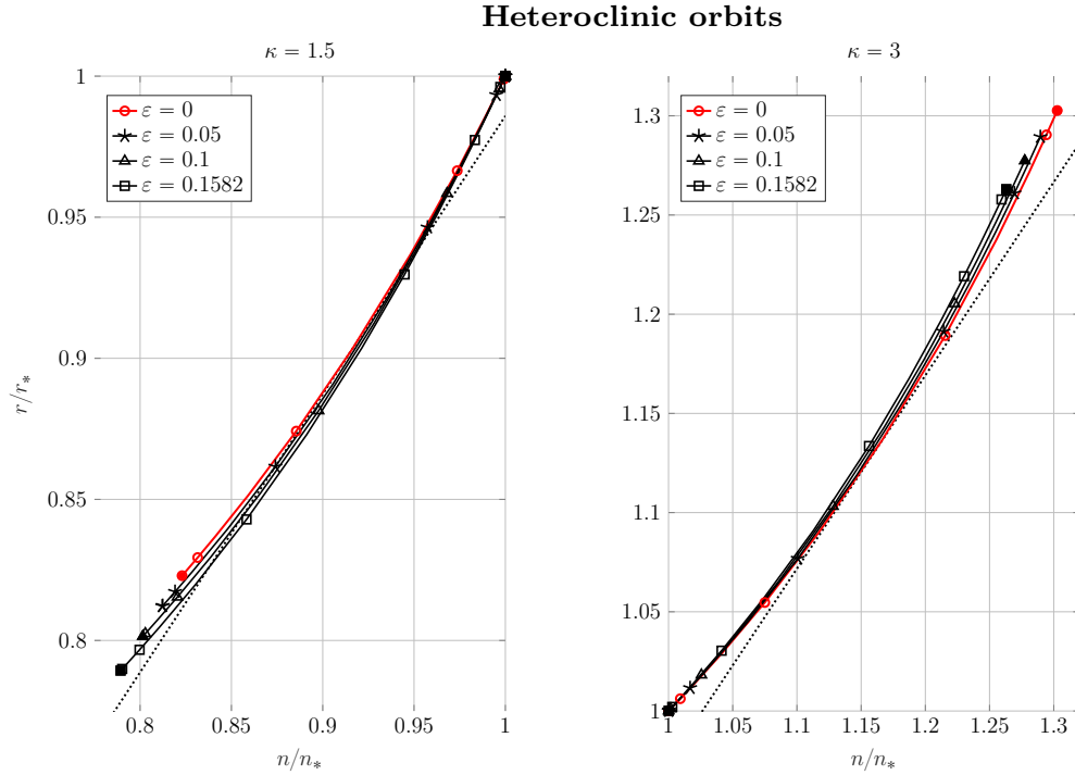
FIGURE 10. Orbits connecting (n_x, r(n_x)) to (1,1) for several values of \epsilon for the \gamma -law (1.5) with exponent \gamma = 2 . The straight line n \mapsto \tau_{\#}(\kappa)n is plotted for reference, and the tangent point with the corresponding orbit is indicated (markers as in Figure 9).
