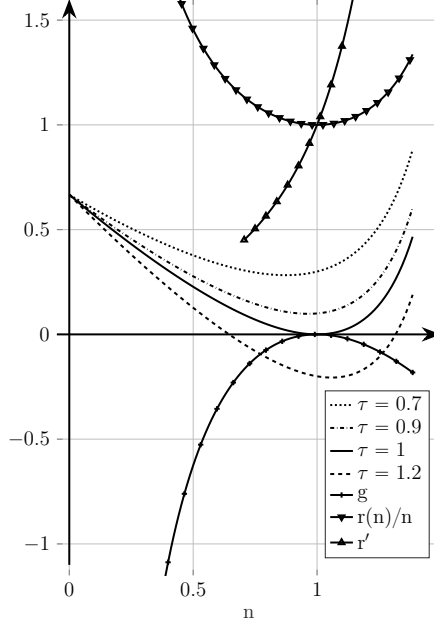
FIGURE 8. Graphs of functions \varphi(n) = r_\kappa(n) - \tau n in the case of \gamma -law (1.5) with \gamma = \kappa = 2 and various choices of \tau . The graph of g_\kappa (with opposite convexity) has been superposed for comparison, as well as the maps n \mapsto r_\kappa(n)/n and n \mapsto r'(n) that intersect at (n_\#, \tau_\#) .
