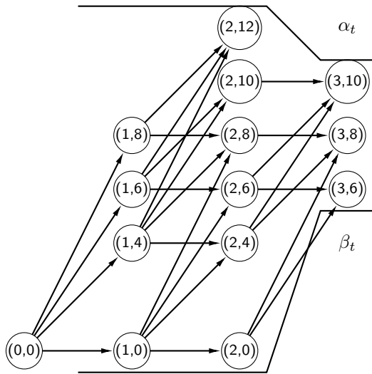
(a) Graphical representation as a knapsack problem
