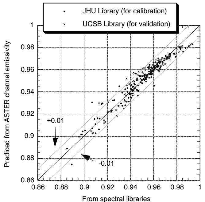
Fig. 2. Predictions of broadband emissivity.
