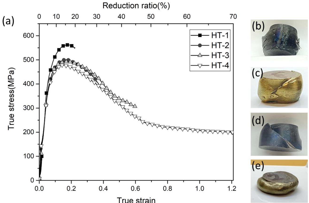
Figure. 8. (a) Stress-strain curve of four specimens tested at 1000 °C with a strain rate of 0.1s -1 and the macroscopic view of deformed samples (b) HT-1, (c) HT-2, (d) HT-3, (e) HT-4.
