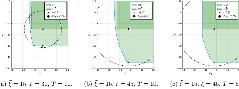
Fig. 2: Plots of the two SST \mathbb{S}(\bar{\xi}) and \mathbb{S}(\xi) , with the points c(\xi, \bar{\xi}) \in \mathbb{S}(\xi) (denoted with a cross) achieving the largest distance to \mathbb{S}(\bar{\xi}) , as well as its projection on \mathbb{S}(\bar{\xi}) (denoted by a diamond). The plots also showcase the circle centered at P_{\mathbb{S}(\bar{\xi})}(c(\xi, \bar{\xi})) with radius 1.1|\bar{\xi} - \xi| .
