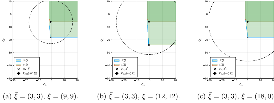
Fig. 3: Plots of the two SST \mathbb{S}(\bar{\xi}) and \mathbb{S}(\xi) , with the points c(\xi, \bar{\xi}) \in \mathbb{S}(\xi) (denoted with a cross) achieving the largest distance to \mathbb{S}(\bar{\xi}) , as well as its projection on \mathbb{S}(\bar{\xi}) (denoted by a diamond). The plots also showcase the circle centered at P_{\mathbb{S}(\bar{\xi})}(c(\xi, \bar{\xi})) with radius 2\|\bar{\xi} - \xi\| .
