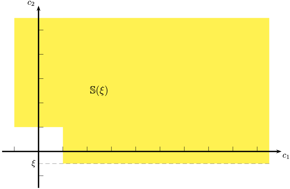
Fig. 1: Sketch of the SST of Example 1.
