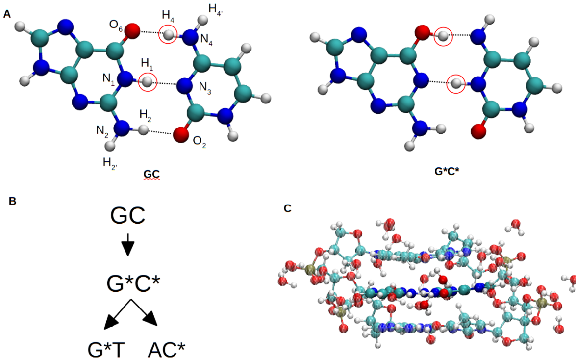
Figure 1: Panel A) Canonical (GC) and tautomeric ( G^*C^* ) forms of the Guanine-Cytosine base pair, with atom numbering. Transferring hydrogen atoms are shown in red circles. Panel B) Schematic representation of the tautomerism and its impact on the replication of DNA, with a GC base pair forming the G^*C^* tautomer and eventually leading to non-standard pairing G^*T or AC^* (A = Adenine and T = Thymine). Panel C) Structure of the 3BP-DNA model extracted from the 1D28 PDB structure 23 with the corresponding crystallographic water molecules.
