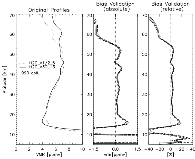
Fig. 1. Left panel: MIPAS H2O_V3O_13 (solid) and H2O_V1/2_5 (dotted) mean profiles. Middle panel: Absolute bias MIPAS (V1/2) – MIPAS (V3O) (solid) with its uncertainty (dashes). Right panel: Relative bias MIPAS (V1/2) – MIPAS (V3O) (solid) with its uncertainty. The uncertainties in the middle and right panel are given in terms of two standard deviations of the mean (dashes).
