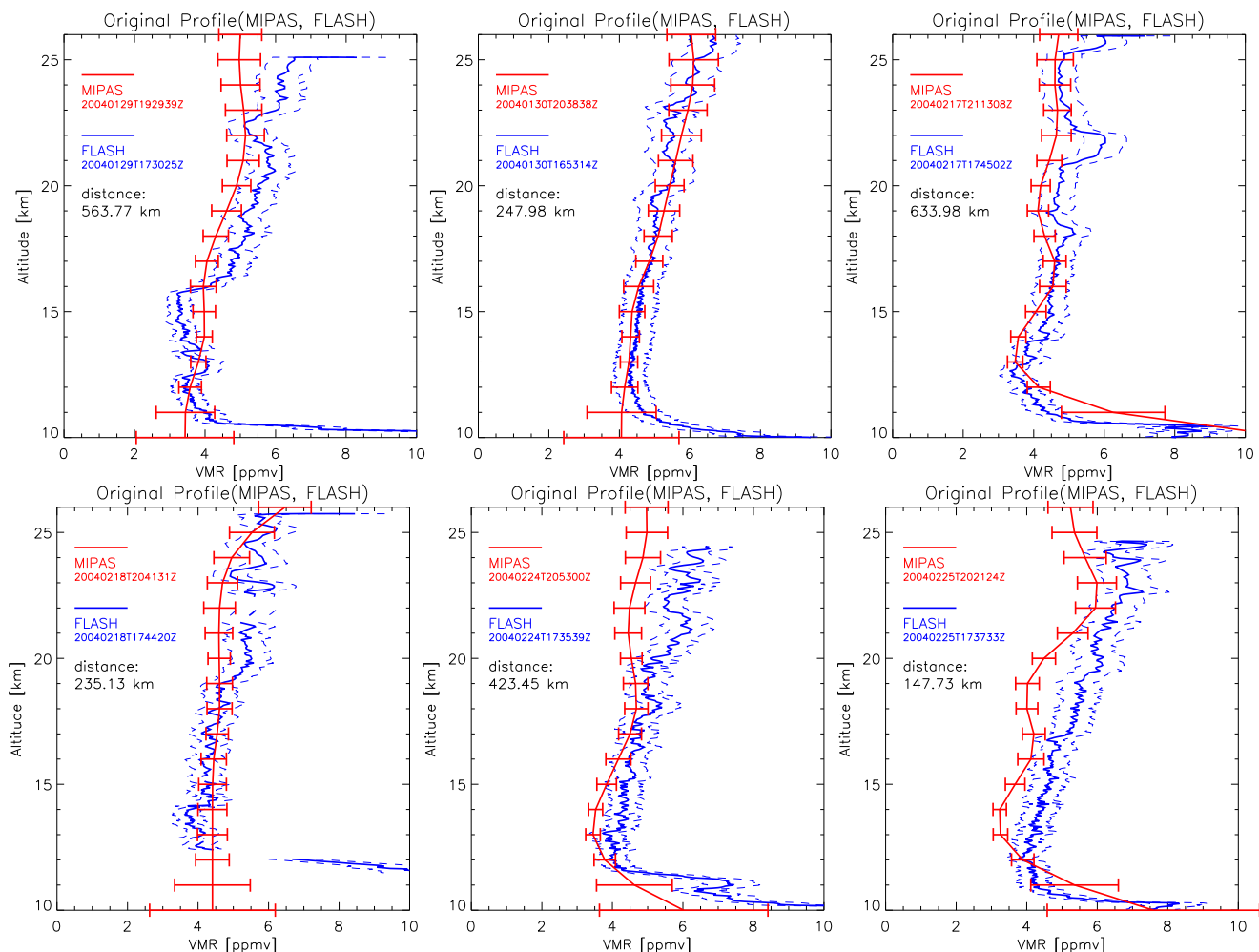
Fig. 22. FLASH-B (blue) and MIPAS (red) H 2 O profiles for six coincidences the dashed lines indicate the error bars of the FLASH-B measurement.
