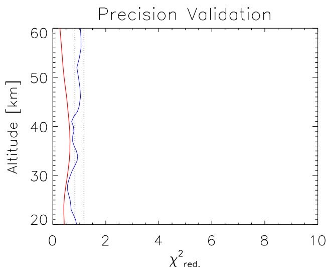
Fig. 17. \chi^2 analysis for precision validation for MIPAS and ground based MIAWARA water vapour measurements recorded in Sodankylä. Blue: MIPAS original profiles. Red: MIPAS profiles smoothed with MIAWARA averaging kernels. For details, see Fig. 3.
