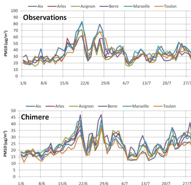
Fig. 4. Observed (upper graph) and modeled (lower graph) daily mean concentrations of \text{PM}_{10} at the 6 measurement sites
