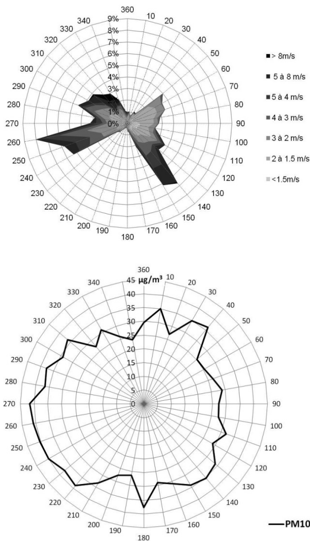
Fig. 2. Wind (top) and PM concentration (bottom) sector plots at Arles for June and July 2006.
