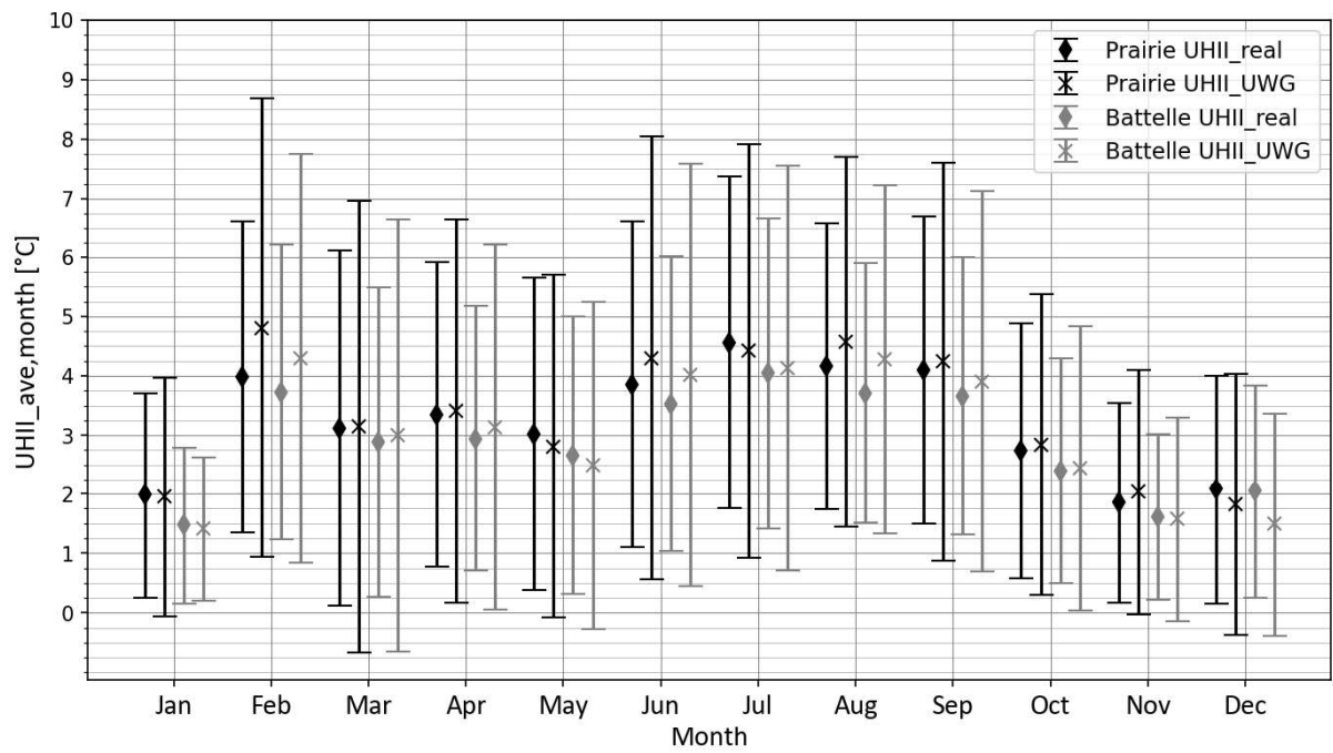
Figure 11: Average monthly UHI (markers) and standard deviation (bars) arising from UWG simulations (UHII_UWG) and from real measurements (UHII_real) for two selected urban weather stations
