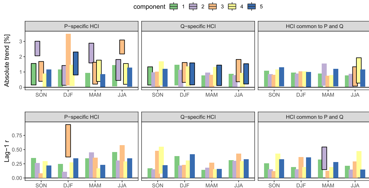
Figure 6. Summary of Hidden Climate Indices properties for all 5 components and 4 seasons. Boxes denote 90% posterior intervals for the absolute trend |\beta| (top) and the lag-1 autocorrelation r = e^{-1/\tau_1} (bottom). Outlined boxes highlight “large” trends and autocorrelations, and correspond to \beta -intervals not containing 0 or r -intervals above 0.1.
