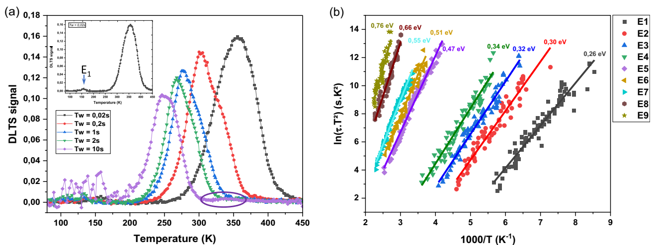
Figure 5. a) DLTS spectra obtained from the analysis of transient for different time windows ( T_w on the graph) in the case of sine Fourier coefficient b_1 . The spectrum for T_w = 0.02 s is displayed in the inset revealing the presence of a small peak denoted E_1 . The purple oval underlines the presence of a broad peak with weak intensity. b) Corresponding Arrhenius plot deduced from the Fourier analysis of the transients at different T_w and for Fourier coefficient. Nine different traps signature are obtained.
