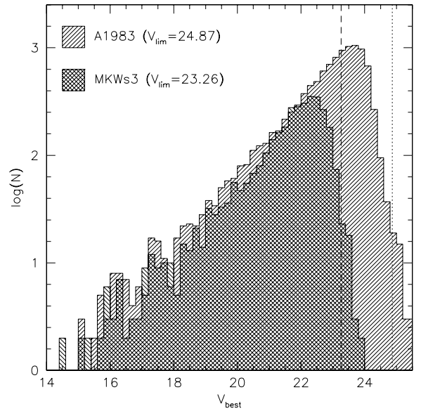
Fig. 10. V -band magnitude histograms for A1983 and MKWs3, compared with the corresponding detection limit magnitudes computed using Eq. (1) (vertical lines).
