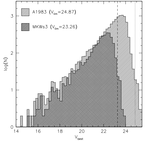
Fig. 10. V -band magnitude histograms for A1983 and MKW3s, compared with the corresponding detection limit magnitudes computed using Eq. (1) (vertical lines).
