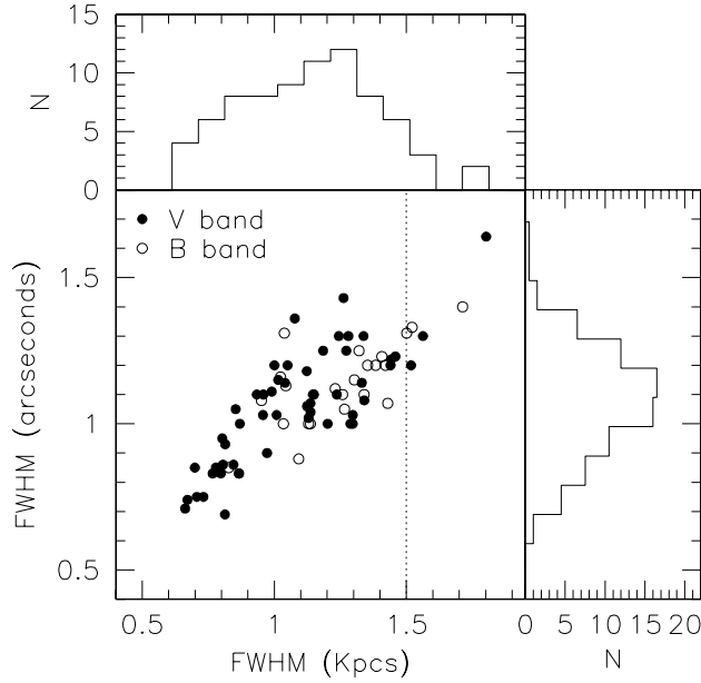
Fig. 8. The FWHM in arcseconds versus the physical size this projects to at the cluster redshift, with the marginal distributions for each, for the WINGS-OPT imaging. Filled and open circles indicate that the best FWHM is achieved in the V and B band, respectively.
