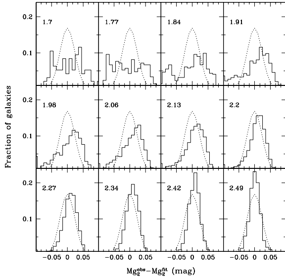
Figure 9. Distribution of residuals relative to the mean Mg_2-\sigma_v relation fitted in Fig. 8, for different values of \log(\sigma_v/\text{km s}^{-1}) (indicated in each panel). The number of galaxies is normalized to the total in each bin of velocity dispersion. The dotted curve (repeated in each panel) is a Gaussian distribution of width equal to the average absolute deviation in the Mg_2-\sigma_v relation (see Table 1).
