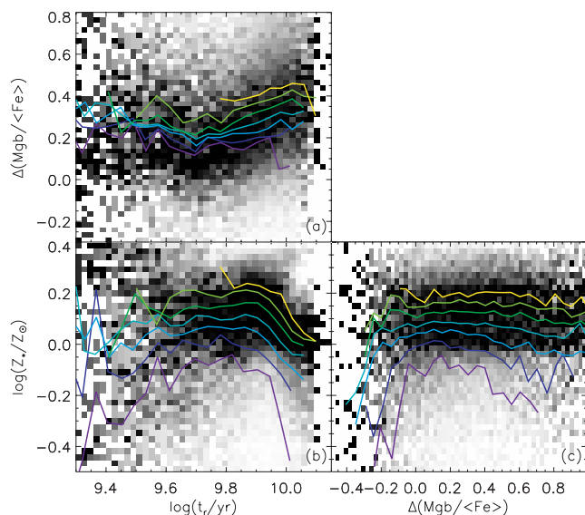
Figure 18. Correlations between stellar metallicity, light-weighted age and \alpha/\text{Fe} -estimator \Delta(\text{Mgb}/\langle\text{Fe}\rangle) . The solid lines represent the median relations for galaxies in different bins of velocity dispersion, centred on \log(\sigma_v/\text{km s}^{-1}) = 1.9, 2, 2.1, 2.2, 2.3, 2.4, 2.5 (increasing from purple to yellow). The grey-scale indicates the density of galaxies with respect to the total at fixed abscissa.
