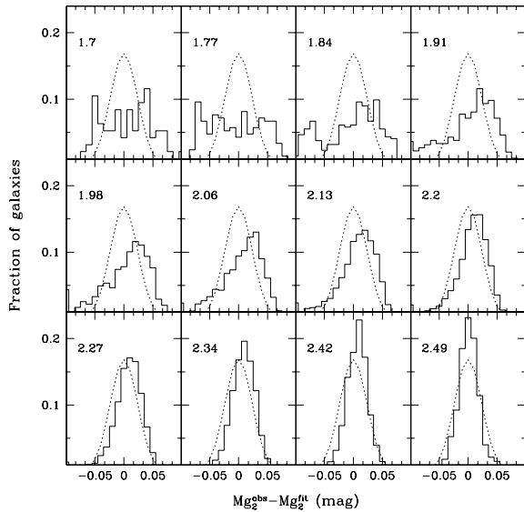
Figure 9. Distribution of residuals relative to the mean Mg_2-\sigma_v relation fitted in Fig. 8, for different values of \log(\sigma_v/\text{km s}^{-1}) (indicated in each panel). The number of galaxies is normalized to the total in each bin of velocity dispersion. The dotted curve (repeated in each panel) is a Gaussian distribution of width equal to the average absolute deviation in the Mg_2-\sigma_v relation (see Table 1).
