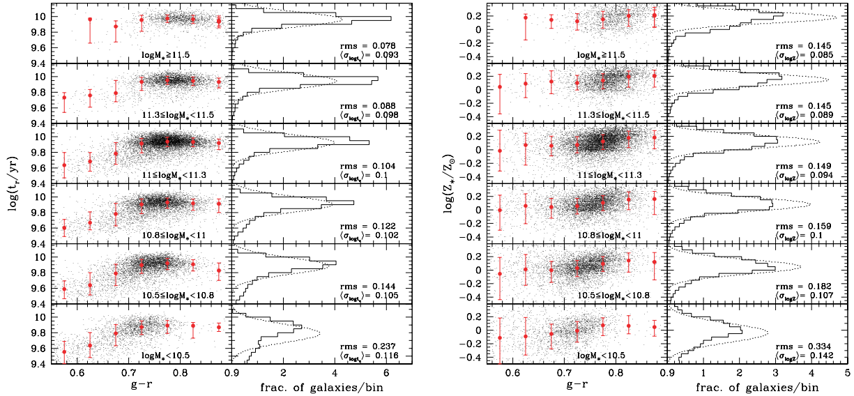
Figure 7. Left-hand panels: distribution in light-weighted age (left-hand plot) and stellar metallicity (right-hand plot) as a function of g - r colour for different bins of stellar mass. The red dots are the median age (metallicity) at fixed colour, while the error bars give the 68 per cent percentile range in the age (metallicity) distribution. Right-hand panels: histogram of light-weighted age (metallicity) compared to a Gaussian (dotted curve) of width equal to the average error on age (metallicity) in each stellar mass bin. In each panel, the rms scatter and the average error in age (metallicity) are also given.
