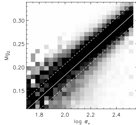
Figure 8. Relation between \text{Mg}_2 index strength (mag) and velocity dispersion \log \sigma_v (\text{km s}^{-1}) for the same sample of early-type galaxies as in Fig. 1. As in Fig. 3, the grey-scale indicates, for each velocity dispersion bin, the relative distribution of galaxies in the different \text{Mg}_2 bins.
