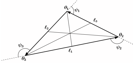
Fig. 1. Definition and convention of triangle variables.
