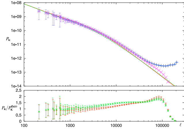
Fig. B.1. Power spectrum of \kappa measured on the 40 lensing pseudo-realization. Lines are the predicted power spectrum using the PD (Peacock & Dodds 1996) (dashed) or haloFit (Smith et al. 2003) prescription for the small scales. Points are the measurements in the simulations, without smoothing (crosses), and with smoothing (xs) to remove the Poisson noise (see text). Bottom panel shows the ratio between the smoothed measured power spectrum and the two predictions using PD (xs) and haloFit (crosses).
