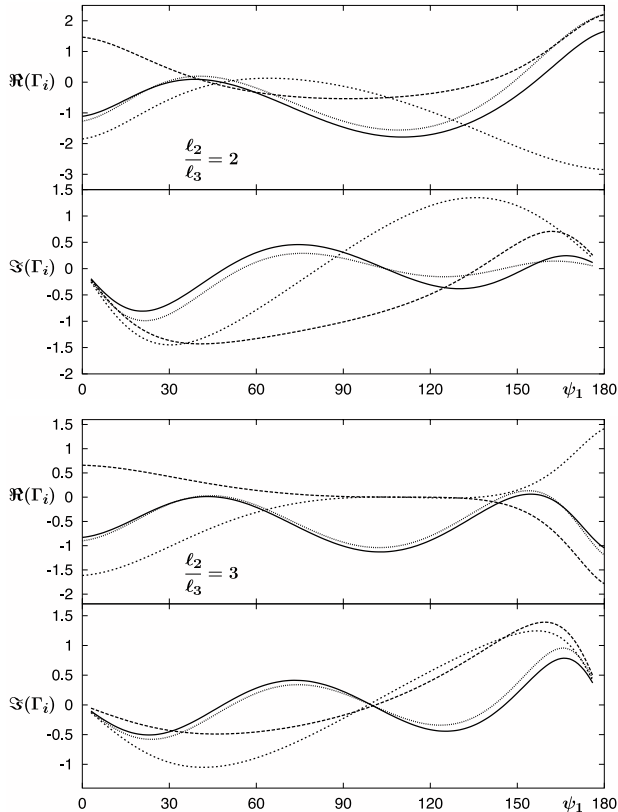
Fig. 4. Same as Fig. 3 but only in the center of mass projection, for sides ratio \ell_2/\ell_3 = 2 (top panel) and \ell_2/\ell_3 = 3 (bottom panel).
