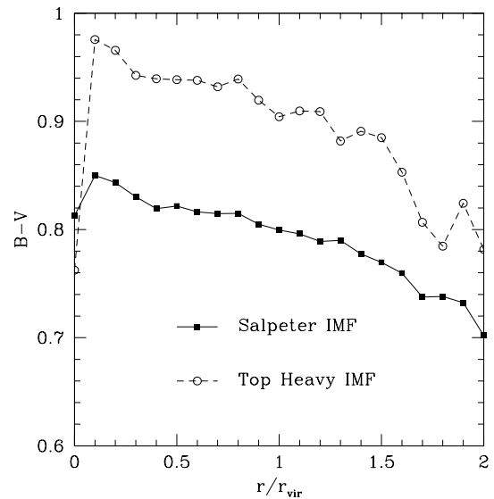
Figure 9. The radial dependence of galaxy colours, averaged over all simulated clusters. In each panel, solid lines with filled squares are for the Sa-IMF, while dashed line with open circles is for the TH-IMF. The reported results are the average over all the simulated clusters.
