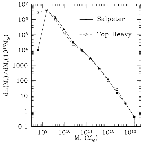
Figure 7. The combined stellar mass function for the galaxies identified within r_{200} of all clusters. The solid and the dashed histograms correspond to the Salpeter and the TH-IMF, respectively.
