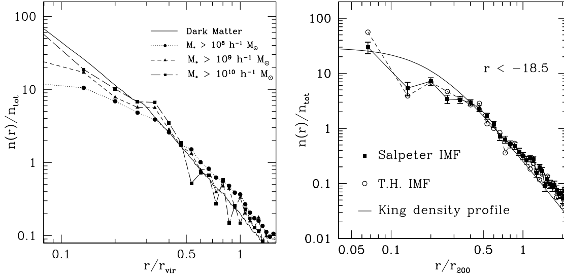
Figure 1. The number density profile of cluster galaxies. Left-hand panel: the profiles of galaxies of different stellar mass, averaged over all clusters, for the runs with Sa-IMF (filled symbols). Shown with the solid curve is the average DM profile. All profiles are normalized to the total number density within the virial radius. Right-hand panel: the number density of galaxies, brighter than r = -18.5 , contained within a given radius, normalized to the total number density found within the r_{200} . Filled squares and open circles are combination of all the simulated clusters, for the Salpeter and for the TH-IMF, respectively. The solid curve is the best-fitting King model to the number density profiles of cluster galaxies from the analysis of RASS-SDSS data by Popesso et al. (2006b), plotted here with arbitrary normalization. Error bars in the simulation profile correspond to Poissonian uncertainties. For reasons of clarity, they have been plotted only for the Salpeter runs.
