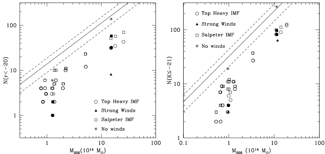
Figure 5. The number of galaxies within clusters above a given luminosity limit. Left-hand panel: results in the r band, compared to the observational best-fitting result from SDSS data by Popesso et al. (2006b). (The dashed lines mark the intrinsic scatter of the observational relation.) Right-hand panel: results in the K band, compared to the observational best-fitting result from 2MASS data by Lin et al. (2004). Symbols for the simulations have the same meaning as in Fig. 4.
