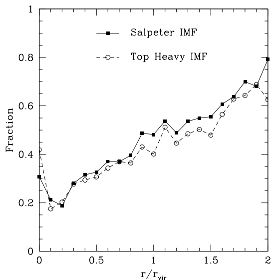
Figure 10. The fraction of galaxies younger than 8.5 Gyr, as a function of cluster-centric distance, in units of r_{\text{vir}} . Symbols and line types have the same meaning as in Fig. 9.
