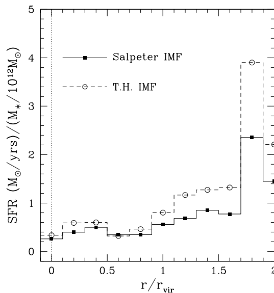
Figure 11. The specific mean SFR, averaged over all the simulated clusters, as a function of the cluster-centric distance. Symbols and line types have the same meaning as in Fig. 9. In the central bin, we have excluded the contribution from the BCGs.
