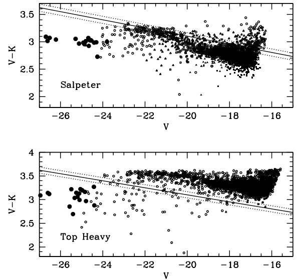
Figure 2. The V - K versus V CMR by combining all the galaxies within the virial radii of the simulated clusters, for the Sa-IMF (top panel) and for the TH-IMF with normal feedback (bottom panel). Straight lines in each panel show the observed CMR relations by Bower et al. (1992), with the corresponding intrinsic standard deviations. Big filled dots mark the BCG of each cluster. Different symbols and colours are used for galaxies having different metallicities. Magenta open circles: Z > 1.5 Z_\odot ; blue filled triangles: 1.5 < Z/Z_\odot < 1 ; red open squares: 1 < Z/Z_\odot < 0.7 ; black open triangles: 0.7 < Z/Z_\odot < 0.4 ; green filled squares: Z < 0.4 Z_\odot .
