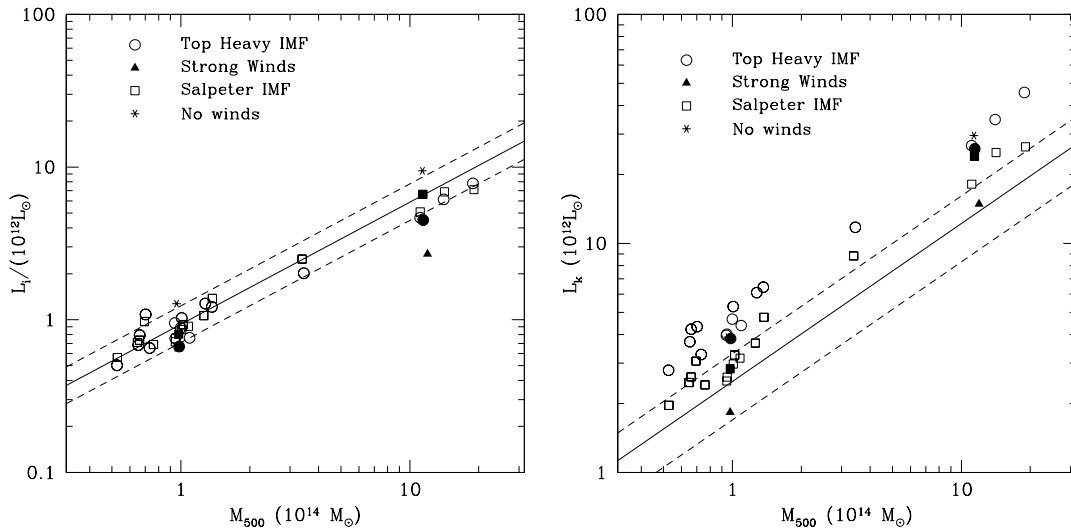
Figure 4. The comparison between simulated and observed relation between mass and luminosity in the i band (left-hand panel) and in the K band (right-hand panel). In each panel, squares are for the Sa-IMF, circles for the TH-IMF with normal feedback, triangles for the TH-IMF with strong feedback and asterisks for the Sa-IMF with no feedback. Filled squares and circles are for the g676 and g51 runs, so as to make clear the effect of changing the feedback strength. The straight solid lines are the best-fitting results from Popesso et al. (2005) for the i band and from Lin et al. (2004) for the K band, with the dashed lines marking the corresponding observational scatter.
