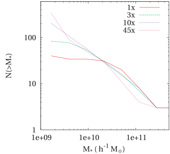
Figure A2. The combined cumulative stellar mass function of the galaxies identified within the virial radii of the three clusters. The four curves correspond to the different resolutions at which the clusters have been simulated. Continuous, long-dashed, short-dashed and dotted curves are for the simulations at progressively increasing resolution. The labels indicate the factor by which mass resolution is increased, with respect to the lowest resolution run (1x).
