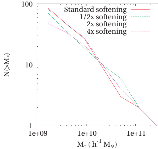
Figure A1. The cumulative stellar mass function of the galaxies identified within the virial radii of the most massive among the three simulated clusters described in the Appendix (see also Borgani et al. 2006). All the simulations have been done at fixed mass resolution, which correspond to an increase by a factor of 10 with respect to the basic resolution (i.e. m_{\text{gas}} \simeq 6.9 \times 10^7 h^{-1} M_{\odot} ; see text). The four curves correspond to the different choices for the gravitational softening. The labels indicate the factor by which the softening has been changed, with respect to the standard choice of 3.5 h^{-1} \text{kpc} .
