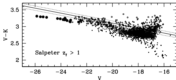
Figure 3. The same as the top panel of Fig. 2, but only including in the computation of the luminosities the star particles having redshift of formation z_f > 1 .
