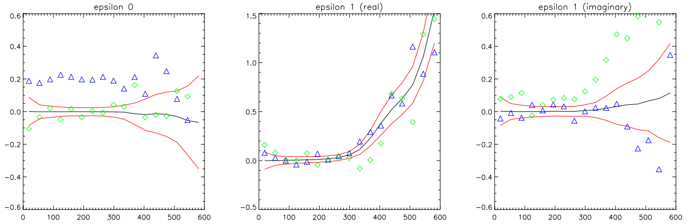
FIG. 4 (color online). D_\ell measured on the WMAP data (V band) [green diamonds]. Blue triangles are the measurements on a simulated map with \epsilon_0 = 0.2 and the red (upper and lower solid) lines are 1\sigma error bars.
