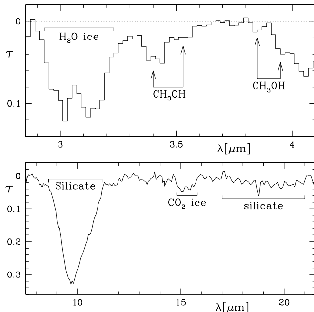
Figure 5. VLT/ISAAC (top, heavily smoothed) and Spitzer /IRS (bottom) spectra of IRAS 05328–6827, expressed in optical depth with respect to the continuum drawn in Fig. 4. There is clear evidence for absorption by ices of \text{H}_2\text{O} , \text{CH}_3\text{OH} and \text{CO}_2 .
