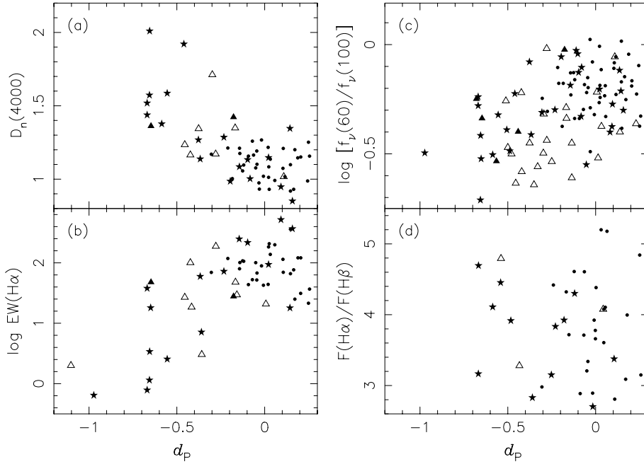
Figure 2. (a) Spectral discontinuity at 4000 Å, (b) H \alpha emission equivalent width, (c) ratio of IRAS f_{\nu}(60\ \mu\text{m}) and f_{\nu}(100\ \mu\text{m}) flux densities and (d) H \alpha /H \beta ratio plotted as a function of perpendicular distance from the mean starburst IRX–UV relation, for the subsets of galaxies for which these observed quantities are available in the sample of Fig. 1. The different symbols have the same meaning as in Fig. 1.
