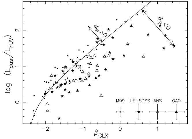
Figure 1. Ratio of far-infrared to ultraviolet luminosity plotted against ultraviolet spectral slope (the IRX–UV diagram). The data points are from the sample compiled in Section 2.1 (median measurement errors for each subsample are indicated in the lower right corner). The solid line shows the mean IRX–UV relation for the 50 starburst galaxies in this sample (equation 2).
