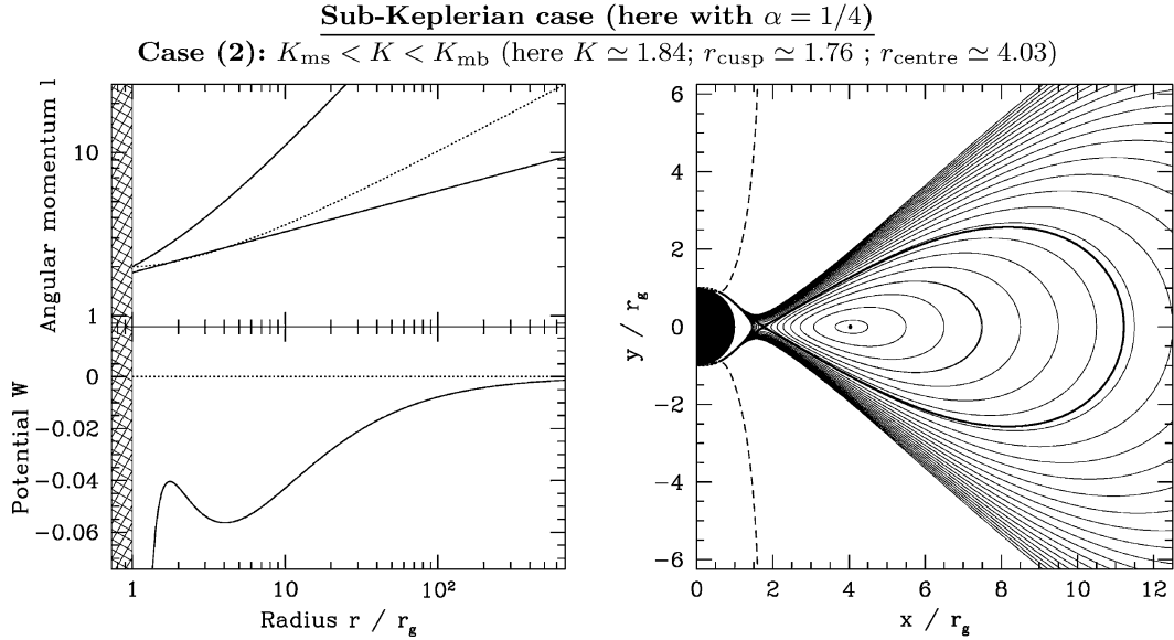
Figure 5. Geometry of the equipotentials: Schwarzschild black hole ( a = 0 ) and extreme Kerr black hole ( a = 1 ). Prograde sub-Keplerian disc. All line styles and notations are identical to those used in Fig. 4 but we have only represented the disc configuration of physical interest, i.e. a finite disc with a centre and a cusp. Schwarzschild black hole: note that, the black hole being non-rotating, a retrograde disc would adopt the same figure of equilibrium. Extreme Kerr black hole: note the scale change in the plots on the right-hand column as compared to the Schwarzschild black hole case or the mildly rotating Kerr black hole case (Fig. 4).
