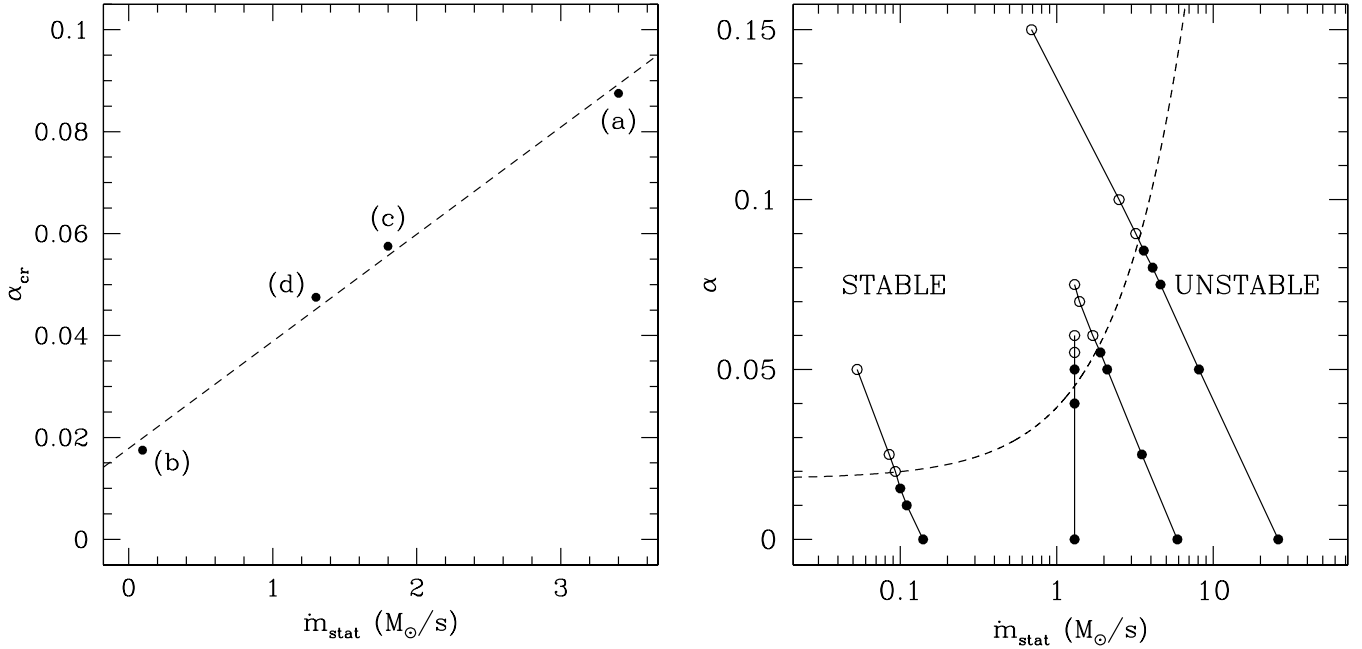
Figure 12. Left-hand panel: the best estimate of the critical slope \alpha_{cr} is plotted as a function of the initial mass flux \dot{m}_{stat} . The four points corresponds to the mean value between models 5a and 6a (set ‘a’), models 3b and 4b (set ‘b’), models 4c and 5c (set ‘c’) and models 2d and 4d (set ‘d’). The dashed line indicates the empirical relation \alpha_{cr} \simeq 0.018 + 0.021(\dot{m}/M_{\odot} s^{-1}) . Right-hand panel: all models (series three) are plotted in the \dot{m}_{stat} – \alpha plane. Filled circles indicate unstable discs and empty circles stable discs. The dashed line separating the stable and unstable discs corresponds to the empirical relation shown in the left-hand panel.
