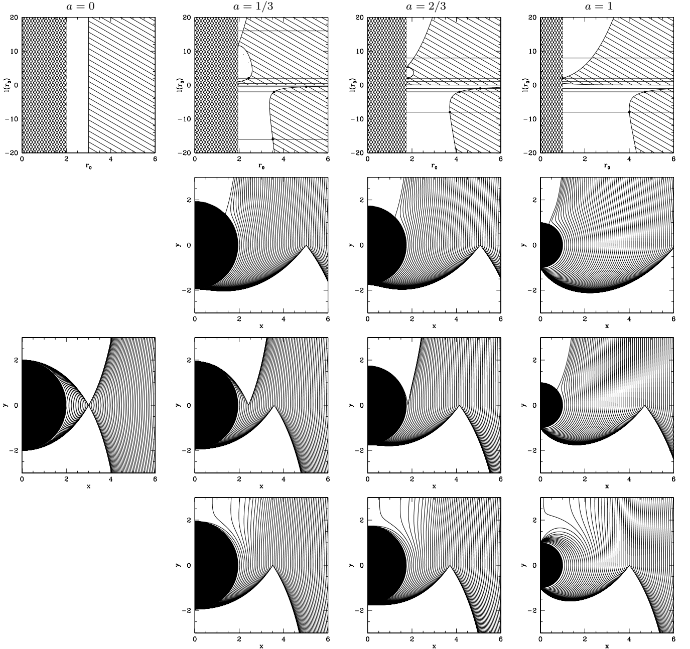
Figure A1. The structure of the von Zeipel's cylinders outside the horizon: each column corresponds to a different value of the spin of the black hole a . The first row shows in the r_0 - l_0 plane the curve \mathcal{P} = 0 (thick line) and the curve \mathcal{Q} = 0 (thin line) as well as the region where \mathcal{Q}/\mathcal{P} < 0 (shaded area), which allows us to predict the behaviour of any cylinder in the vicinity of the equatorial plane (see text). The interior of the horizon has been shaded with hatched lines. For each value of a , the von Zeipel's cylinders are shown in the x - y plane for l_{\text{eq}}(r_0) = \pm 0.5 for a = 1/3 (respectively, \pm 1 for a = 2/3 and a = 1 ) in the second row, for l_{\text{eq}}(r_0) = \pm 2 in the third row and for l_{\text{eq}}(r_0) = \pm 16 for a = 1/3 (respectively, \pm 8 for a = 2/3 and a = 1 ) in the fourth row. The corresponding distributions of l_{\text{eq}}(r_0) are indicated in the first row as an horizontal thick line. In the case where there is a critical cylinder, it has been plotted with a thick line in the x - y plane and the corresponding (r_0, l_0) values have been indicated with a big dot in the r_0 - l_0 plane. For the second, third and fourth rows, the x - y plane is divided in two regions: y \geq 0 corresponds to prograde rotation ( l_{\text{eq}} > 0 ) and y \leq 0 to retrograde rotation [ l_{\text{eq}}(r_0) \leq 0 ]. In the first column ( a = 0 , non-rotating black hole), the cylinders are independent of the distribution l_{\text{eq}}(r_0) .
