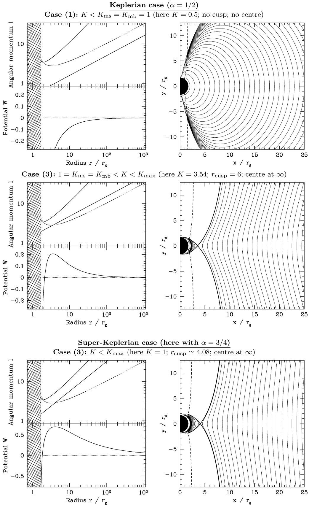
Figure 4 – continued . Keplerian and super-Keplerian cases.
