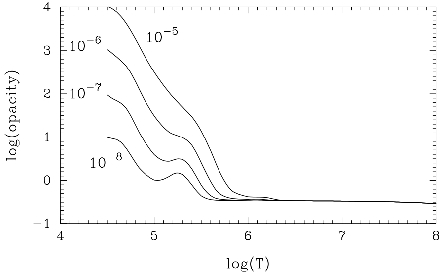
Fig. 1. Opacity as a function of temperature for four values of the density as indicated, and for a composition of X = 0.7 and Z = 0.03 . Quantities are given in cgs units.
