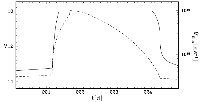
Fig. 9. Optical outburst (dashed line) and the accretion rate when the inner region is assumed to be optically thin (solid) representing the X-ray emission. The inner disc is assumed to be truncated during quiescence ( \mu_{30} = 2 , see Eq. (6)). During outburst the X-ray emission is suppressed whereas the calculations predict increased X-ray emission for 0.5–1 d at the beginning and end of the outbursts.
