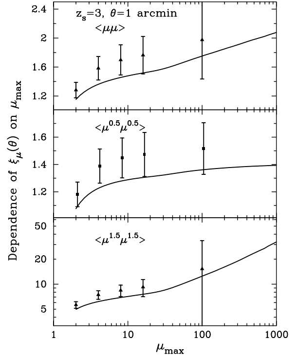
Figure 5. Dependences of the magnification 2PCF amplitude on the maximum magnification cut-off used in the evaluations. For the magnification correlation parametrized as \langle \delta\mu^p \delta\mu^p \rangle , the three panels show the results for p = 1, 0.5 and 1.5 , respectively. The source redshift z_s = 3 and the separation angle \theta = 1 arcmin are considered. All the curves are normalized by the predictions derived from the weak lensing approximation ( \mu \approx 1 + 2\kappa ). As discussed in Section 4, it is expected that the 2PCF amplitude diverges for p \geq 1 for the limiting case \mu_{\max} \rightarrow \infty , while it remains finite for p < 1 (see equation 24). This is verified by the halo model as well as by the simulation.
