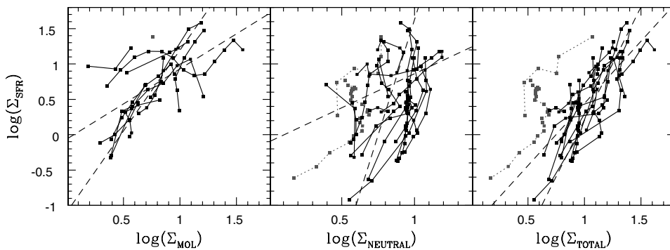
Figure 10. Star formation rate density as a function of molecular gas density (left), neutral gas density (middle) and total gas density (right); units are M_\odot \text{pc}^{-2} \text{Gyr}^{-1} for the SFR and M_\odot \text{pc}^{-2} for the gas (where the He fraction has been accounted for). The data are smoothed to the H I resolution. The solid curves connect points within the same galaxy. The dashed lines are the two regression fits in each case (see the text); the galaxies NGC 3031 and 4258 (indicated by the dotted curves) are excluded from the fit.
