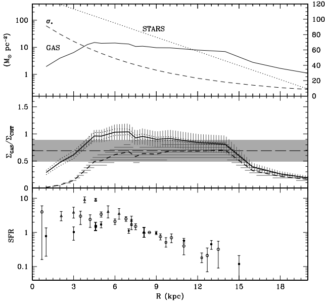
Figure 7. Gas, stars and star formation in the Milky Way disc. Upper panel, observed profiles of the total gas surface density (solid curve, \text{H}_2 + \text{H I} , increased by 40 per cent to include He contribution, the \text{H}_2 being derived from CO with a metallicity-dependent conversion factor), the stellar profile (dotted curve exponential, with scalelength of 2.5 kpc and normalized to 42 M_\odot \text{pc}^{-2} in the solar neighbourhood), and the stellar radial velocity dispersion (dashed curve, calculated according to equations 7 and 8, in \text{km s}^{-1} as indicated on the right axis). Middle panel, profile of the gas surface density to the critical density for two cases: first (dashed curve within horizontally hatched area, indicating the uncertainties on gas values), using equation (4) for \Sigma_{\text{crit}} (i.e. by taking into account only the gas velocity dispersion, assumed here to be 6 \text{ km s}^{-1} at all radii); secondly (solid curve within vertically hatched area, indicating the uncertainties on gas values) using equation (6) for \Sigma_{\text{crit}} (i.e. including the contribution of the stellar disc to the instability criterion). The shaded area indicates the value 0.69 \pm 0.20 that Martin & Kennicutt (2001) found for the star formation threshold in their sample of galactic discs. Bottom panel, SFR profile in the Milky Way (from various tracers), normalized to its value in the solar neighbourhood.
