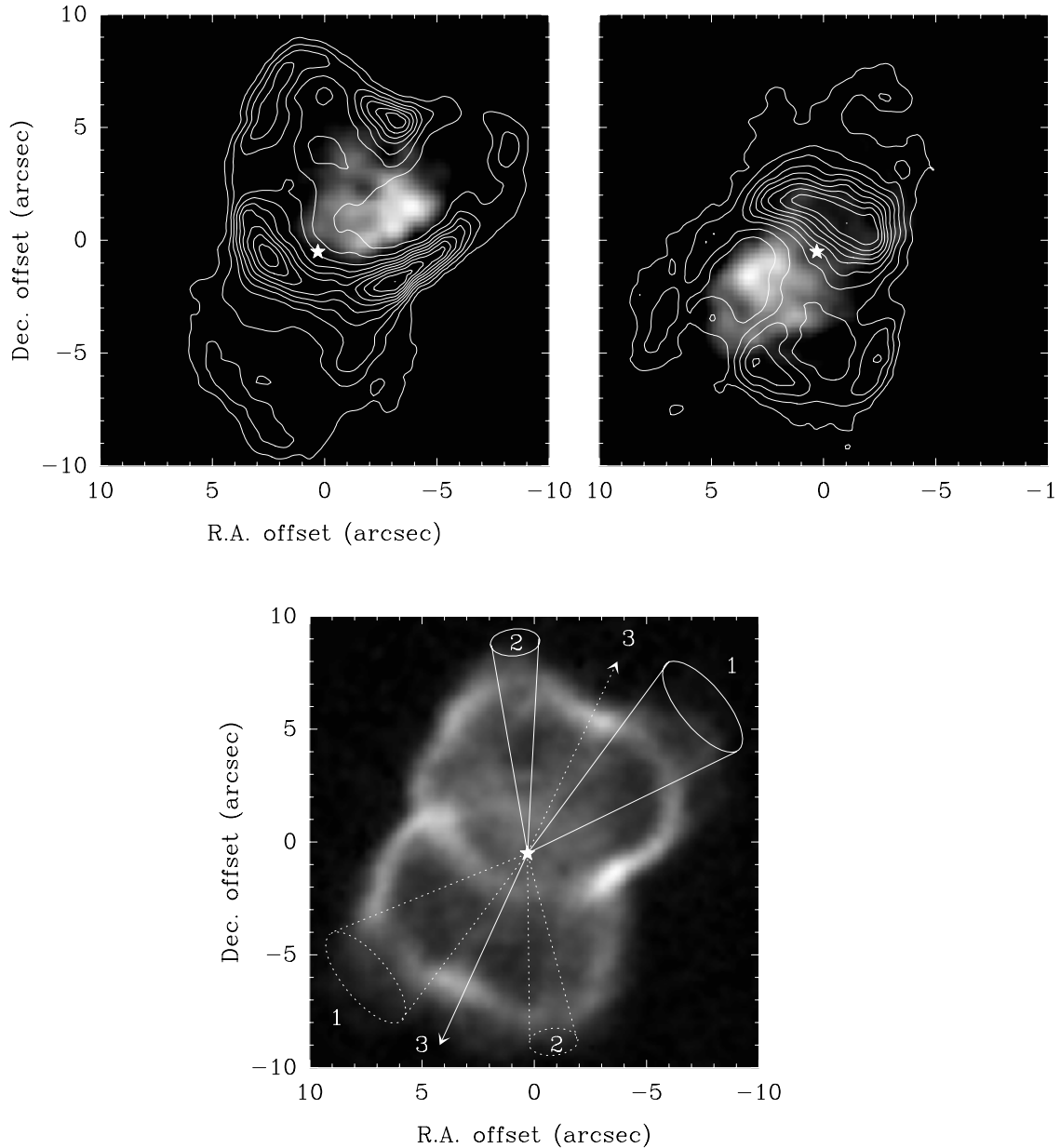
Fig. 10. Identification of the outflow axes in NGC 7027. The bottom panel shows the three outflow axes identified in the H 2 channel maps, superposed on the velocity integrated H 2 emission. The outflow axis labelled 1 can also be identified in the integrated image. The top panel shows the H 2 channel maps (contours) at intermediate velocities (10 and 40 km s -1 in the left and right panels, respectively) superposed on the extreme velocity channels of the Br \gamma emission (-30 and 80 km s -1 respectively).
