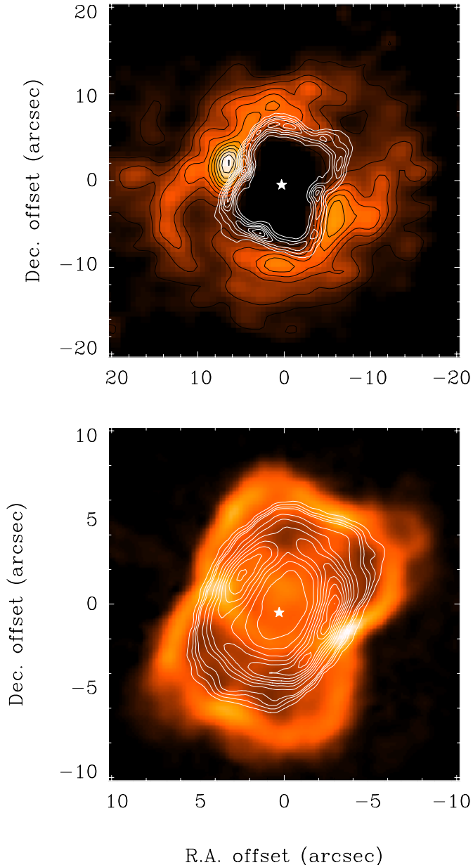
Fig. 7. Upper panel: comparison of the channel map at the systemic velocity ( 25 \text{ km s}^{-1} ) in the CO(1-0) line (from Graham et al. 1993b) (grey scale) with that in the 1-0 S(1) H 2 line at 4712.9 \text{ cm}^{-1} (contours). The channel widths are 5 \text{ km s}^{-1} . Lower panel: comparison of the velocity integrated H 2 line emission with the Br \gamma emission (contours). The offsets are given with respect to the central star (shown as a filled star symbol).
