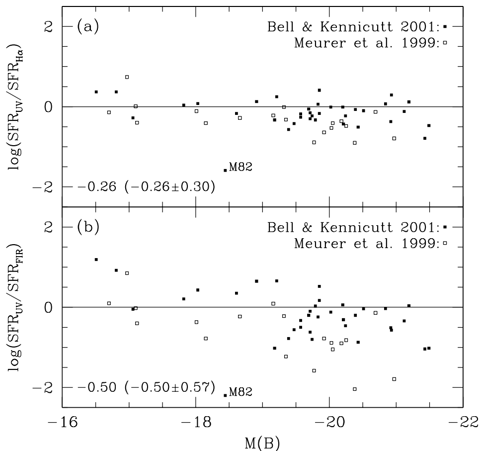
Figure 2. Logarithmic difference between \text{SFR}_{\text{UV}} , \text{SFR}_{\text{H}\alpha} and \text{SFR}_{\text{FIR}} (equations 1, 3 and 4) plotted against the absolute rest-frame B magnitude for the galaxies with \text{H}\alpha , UV (1600 \text{\AA} ) and IRAS 60- and 100- \mu\text{m} flux measurements in the samples of Bell & Kennicutt (2001; solid squares) and Meurer et al. (1999; open squares). In each panel, the median \Delta\log(\text{SFR}) offset for galaxies with M(b_J) < -19 is indicated along with the associated mean offset and the rms scatter (in parentheses).
