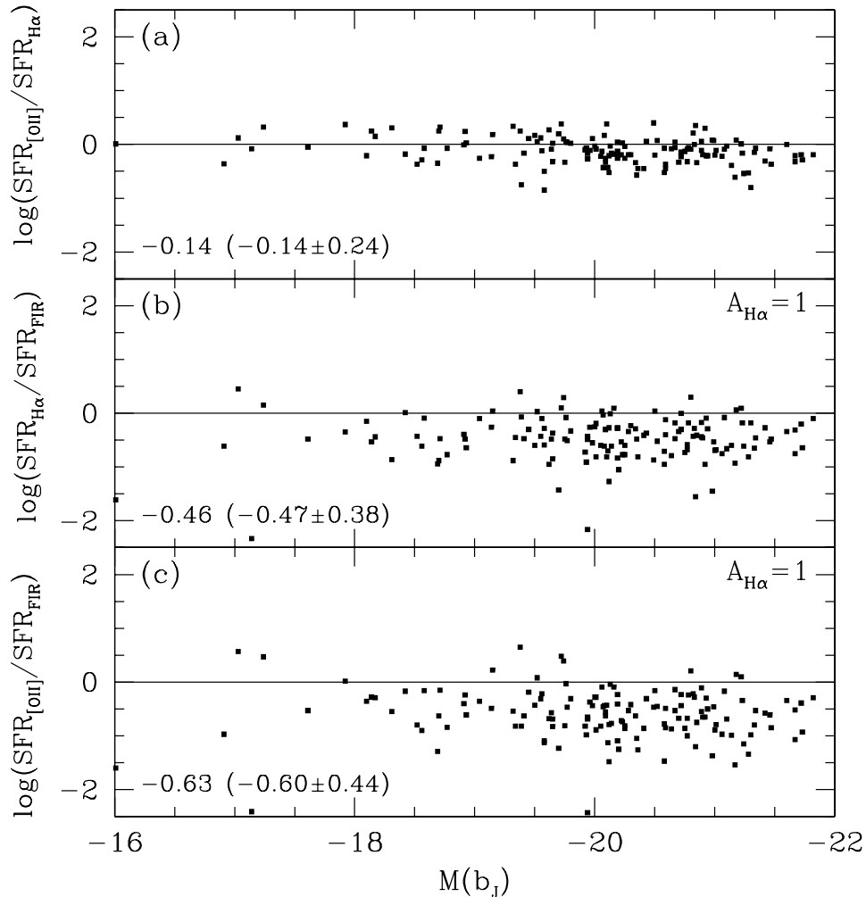
Figure 1. Logarithmic difference between \text{SFR}_{\text{H}\alpha} , \text{SFR}_{[\text{O II}]} and \text{SFR}_{\text{FIR}} (equations 1, 2 and 4) plotted against the absolute rest-frame b_j magnitude for the 149 SAPM galaxies with fluxes and equivalent widths of \text{H}\alpha , [\text{O II}] , and one or both of [\text{N II}] and [\text{S II}] , and IRAS 60- and 100- \mu\text{m} fluxes. We have applied a standard attenuation correction of A_{\text{H}\alpha} = 1 mag to \text{SFR}_{\text{H}\alpha} and \text{SFR}_{[\text{O II}]} . In each panel, the median \Delta \log(\text{SFR}) offset for galaxies with M(b_j) < -19 is indicated along with the associated mean offset and the rms scatter (in parentheses).
