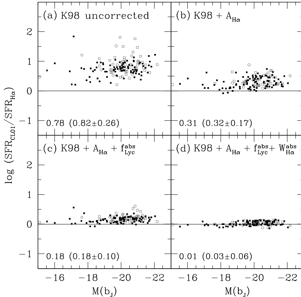
Figure 6. Breakdown of the difference between the CL01 SFR estimates and \text{SFR}_{H\alpha} plotted against the absolute rest-frame b_j magnitude for the 149 SAPM galaxies with fluxes and equivalent widths of H\alpha , [\text{O II}] , and one or both of [\text{N II}] and [\text{S II}] , and IRAS 60- and 100- \mu\text{m} fluxes. Symbols are as described in Fig. 3. (a) Comparison of the CL01 SFRs with those derived from equation (1), before applying any correction for H\alpha attenuation. (b) After correcting the H\alpha -derived SFRs of individual galaxies using the estimated attenuations shown in Fig. 5. (c) After further correction for the fraction of ionizing photons absorbed by dust in H II regions. (d) After further correction for stellar absorption. In each panel, the median \Delta \log(\text{SFR}) offset for galaxies with M(b_j) < -19 is indicated along with the associated mean offset and the rms scatter (in parentheses).
