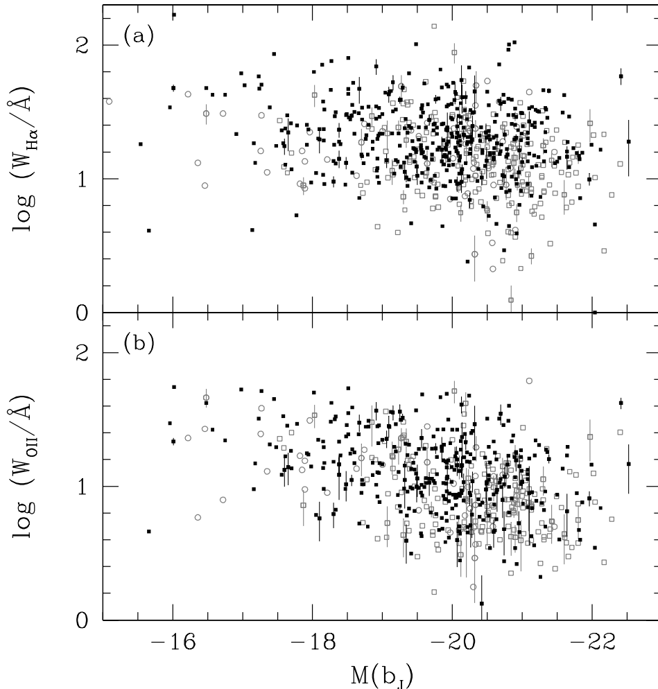
Figure 8. H\alpha and [O\text{II}] rest-frame emission equivalent widths of the 705 SAPM galaxies with fluxes and equivalent widths of H\alpha , [O\text{II}] , and one or both of [N\text{II}] and [S\text{II}] plotted against the absolute rest-frame b_J magnitude. For clarity, only one in seven observational error bars are shown.
