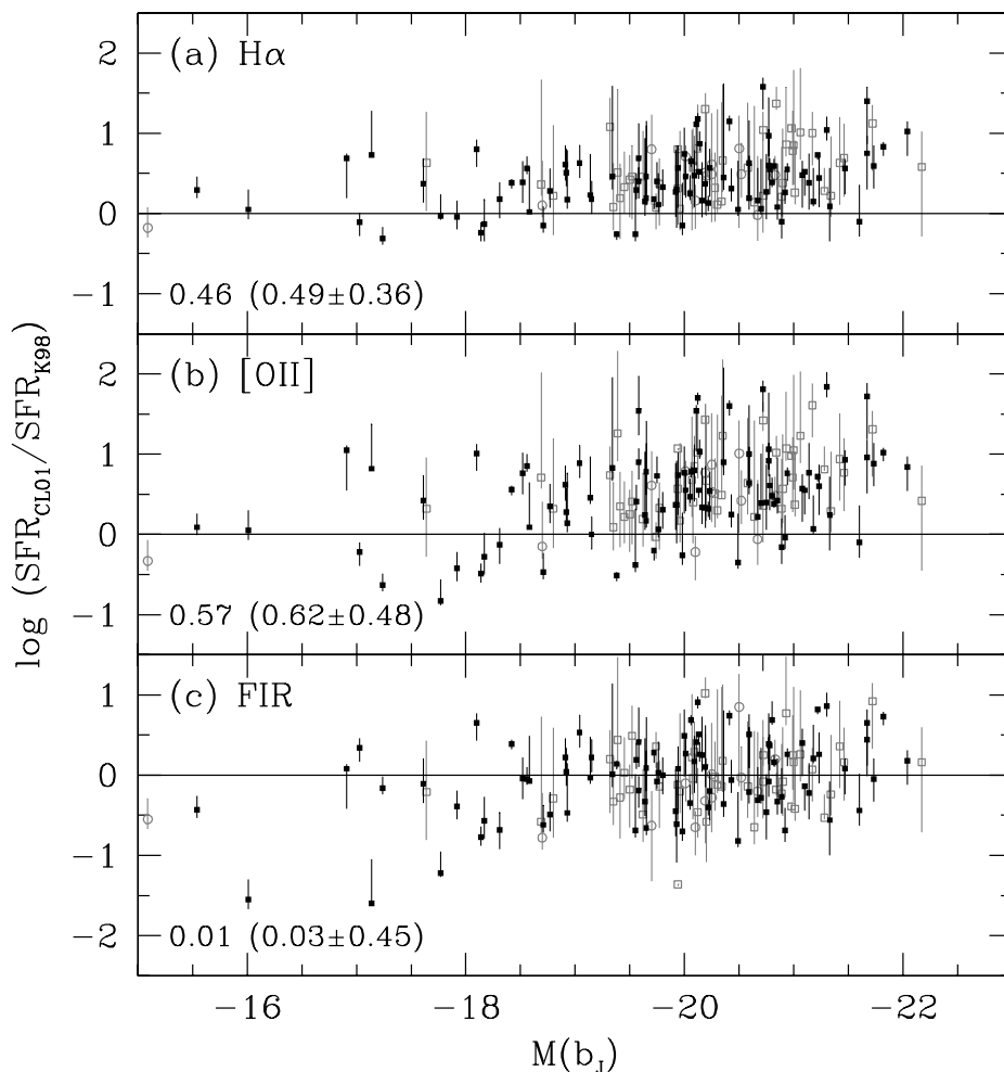
Figure 3. Logarithmic difference between the CL01 SFR estimates and (a) \text{SFR}_{H\alpha} , (b) \text{SFR}_{[\text{O II}]} and (c) \text{SFR}_{\text{FIR}} (equations 1, 2 and 4) plotted against the absolute rest-frame b_j magnitude for the 149 SAPM galaxies with fluxes and equivalent widths of H\alpha , [\text{O II}] , and one or both of [\text{N II}] and [\text{S II}] , and IRAS 60- and 100\text{-}\mu\text{m} fluxes. The CL01 models are required to fit the observed luminosities and equivalent widths of the optical emission lines and the absolute b_j magnitude. The filled squares represent galaxies with measurements of all four optical lines, the open circles galaxies with H\alpha , [\text{O II}] and [\text{N II}] measurements, and the open squares galaxies with H\alpha , [\text{O II}] and [\text{S II}] measurements. The error bars indicate the uncertainties in the SFRs derived using the CL01 model, as discussed in Section 4.2. We have applied a standard attenuation correction of A_{H\alpha} = 1 mag to \text{SFR}_{H\alpha} and \text{SFR}_{[\text{O II}]} . In each panel, the median \Delta\log(\text{SFR}) offset for galaxies with M(b_j) < -19 is indicated along with the associated mean offset and the rms scatter (in parentheses).
