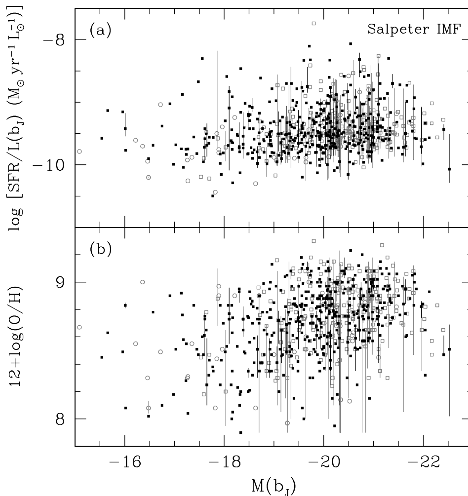
Figure 7. Estimated SFRs and gas-phase oxygen abundances of the 705 SAPM galaxies with fluxes and equivalent widths of H\alpha , [O\ II] , and one or both of [N\ II] and [S\ II] plotted against the absolute rest-frame b_J magnitude. Symbols are as described in Fig. 3. (a) Star formation rate per unit absolute b_J luminosity. (b) Gas-phase oxygen abundance [ 12 + \log(O/H)_\odot \approx 8.8 ]. For clarity, only one in seven error bars are shown to indicate the uncertainties in the SFRs and gas-phase oxygen abundances derived using the CL01 model (as discussed in Section 4.2).
