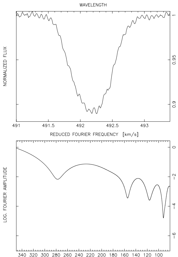
Fig. 1. Mean spectrum for the He I 4921 line (TBL, 2000) (top) and its Fourier transform (bottom).
