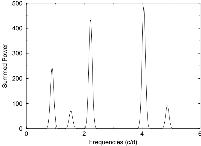
Fig. 5. Power summed across the line profile obtained with the Least Squares method for He I 6678 in 1998.
