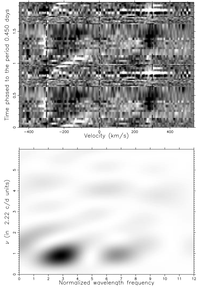
Fig. 8. FDI applied to He I 6678 line. Top: time evolution of residuals in 1998 folded modulo f = 2.2 \text{ c d}^{-1} , after pre-whitening the frequency 4.05 \text{ c d}^{-1} . Bottom: corresponding two dimensional Fourier spectrum of the variations.
