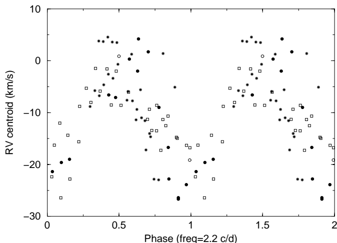
Fig. 10. RV variation of the centroid of the He I 6678 line folded modulo f = 2.2 \text{ c d}^{-1} and with T_0 = 2450624.0 for 1997, 1998 and 2001. Symbols are: filled circles for OHP 1997, open squares for OHP 1998, stars for LNA 2001 and open circles for TBL 2001.
