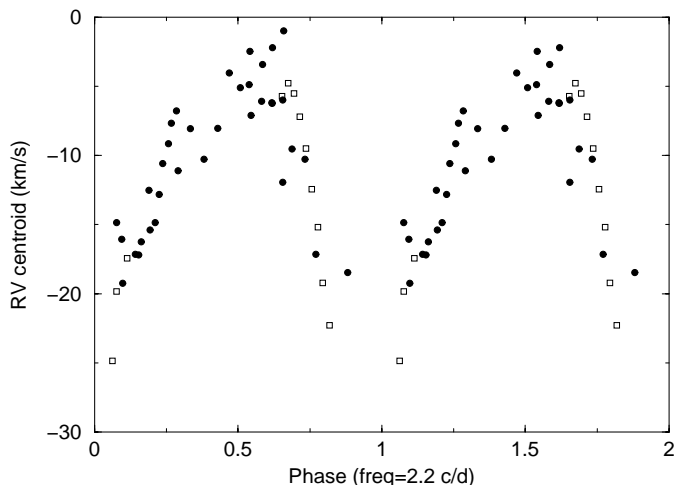
Fig. 11. RV variation of the centroid of the He I 4921 line folded modulo f = 2.2 \text{ c d}^{-1} and with T_0 = 2451715.0 over 2000 and 2001. Symbols are: filled circles for TBL 2000 and open squares for FEROS 2001.
