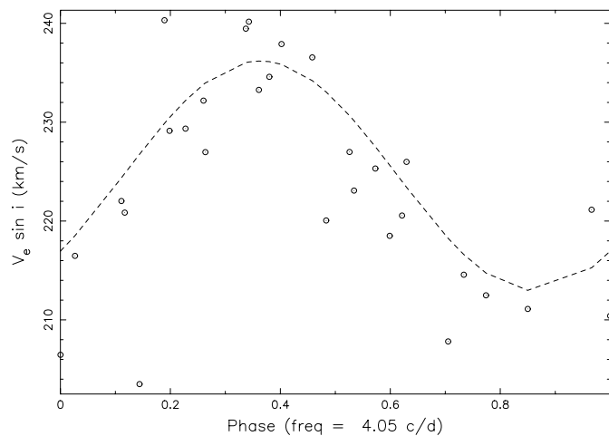
Fig. 13. First minima of the Fourier transform of each He I 6678 line profiles in 1998 folded modulo f = 4.05 \text{ c d}^{-1} and with T_0 = 2450969.0 . The frequency f = 2.22 \text{ c d}^{-1} has been filtered out.
