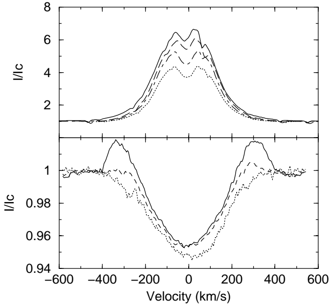
Fig. 4. Upper panel: mean H\alpha line profile. Lower panel: mean He I 6678 line profile. Solid line for 1997, long dashed line for 1998, dot-dashed line for 2000 and dotted line for 2001.
