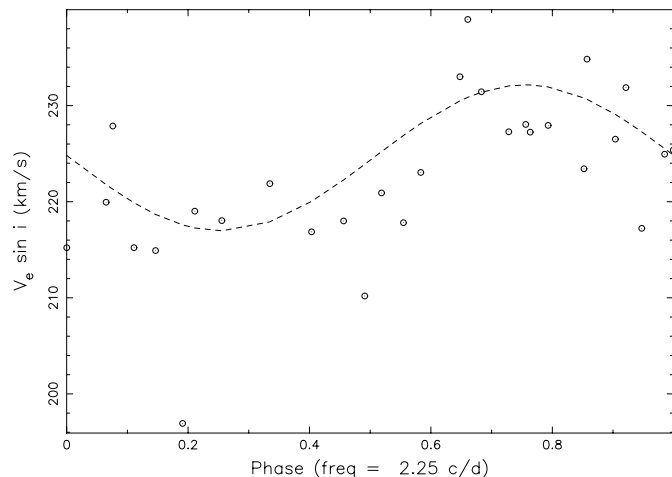
Fig. 12. First minima of the Fourier transform of each He I 6678 line profiles in 1998 folded modulo f = 2.25 \text{ c d}^{-1} and with T_0 = 2450969.0 . The frequency f = 4.05 \text{ c d}^{-1} has been filtered out.
