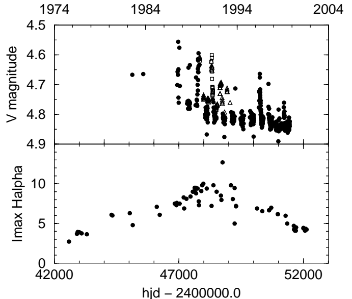
Fig. 2. Correlation between the long-term variation of V band magnitude and the H\alpha intensity. Upper panel: filled circles for Percy et al. (2001), open triangles for Hipparcos data and open squares for Adelman (1992) data. Lower panel: values of I_{\text{max}} taken from Andrillat & Fehrenbach (1982), Banerjee et al. (2000), Buil (2000), Fontaine et al. (1982), Lacy (1977), Hanuschik et al. (1995), Hummel et al. (1995), Peters (1987, 1988a,b,c, 1989a,b, 1990, 1991b,c, 1992, 1994), Slettebak & Reynolds (1978) and this paper.
