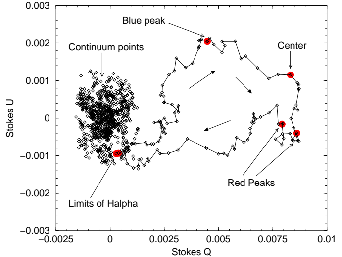
Fig. 15. Polarization across the H\alpha line of 66 Oph in the Q-U plane. Q and U are given in percent. The arrows indicate the increasing wavelength across the line profile. Center, V and R emission peaks are indicated as well as continuum points. The apparent duplicity of the red peak is due to a telluric absorption line.
