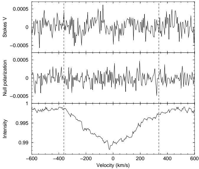
Fig. 14. Example of circularly polarized (Stokes V , upper panel) and unpolarized (lower panel) mean stellar profile of 66 Oph. The null profile is shown in the middle panel.
