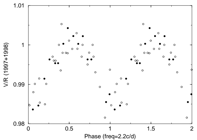
Fig. 9. V/R variation for the He I 6678 line in 1997 and 1998 folded modulo f = 2.2 \text{ c d}^{-1} and with T_0 = 2450624.0 . Symbols are: open circles for 1997 data and filled circles for 1998 data. 1997 data have been shifted by -0.0046 (see text).
