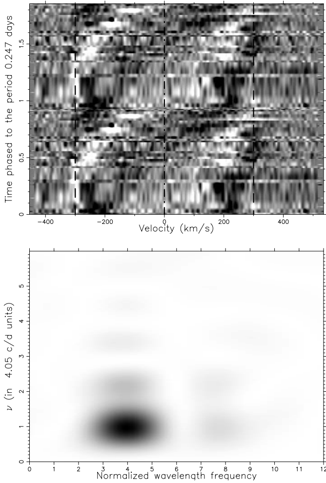
Fig. 7. FDI applied to He I 6678 line. Top: time evolution of residuals in 1998 folded modulo f = 4.05 \text{ c d}^{-1} , after pre-whitening the frequency 2.25 \text{ c d}^{-1} . Bottom: corresponding two dimensional Fourier spectrum of the variations.
