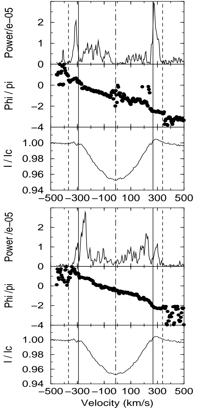
Fig. 6. Line profile variations of He I 6678 in 1998 corresponding to the two detected frequencies 2.22 \text{ c d}^{-1} (upper figure) and 4.05 \text{ c d}^{-1} (lower figure). In each figure power distribution is shown in the upper panel, phase distribution in the middle panel and mean line profile in the lower panel. The vertical lines symbols are: dotted-dashed line for the stellar radial velocity, solid line for the \pm V \sin i extension and dashed lines for the extreme limits of power extension of the two frequencies.
