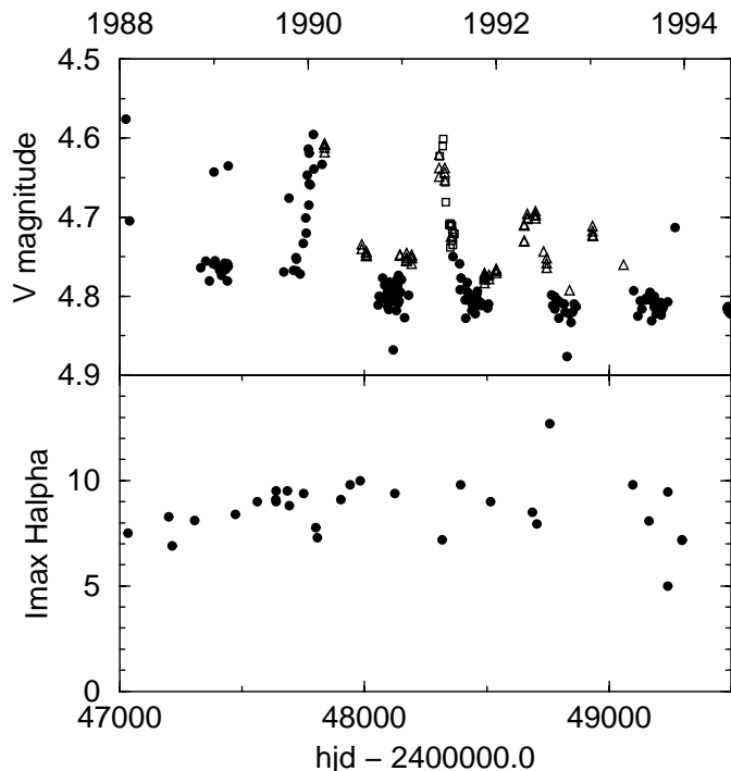
Fig. 3. Correlation between the V band magnitude and the H \alpha intensity during the period of great activity of the star. Symbols and references are the same as in Fig. 2.
