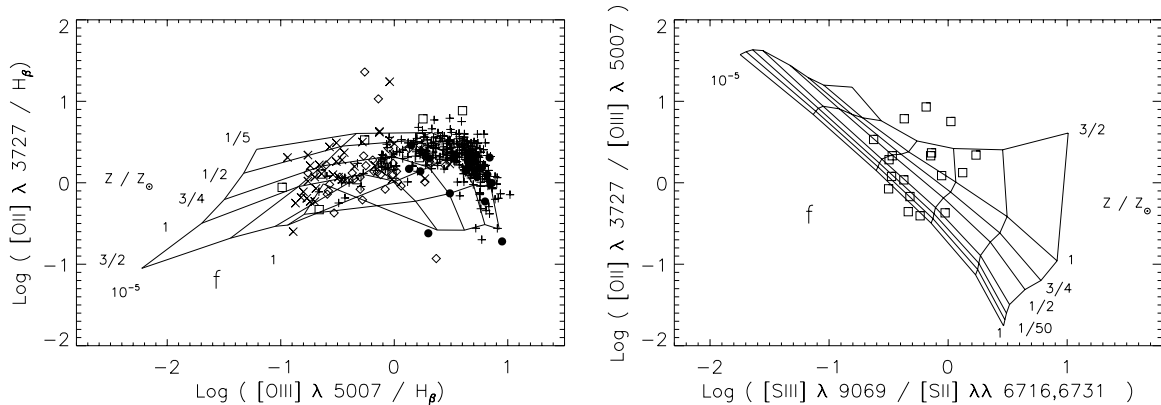
Fig. 2. Same as Fig. 1 for line ratios sensitive to reddening
