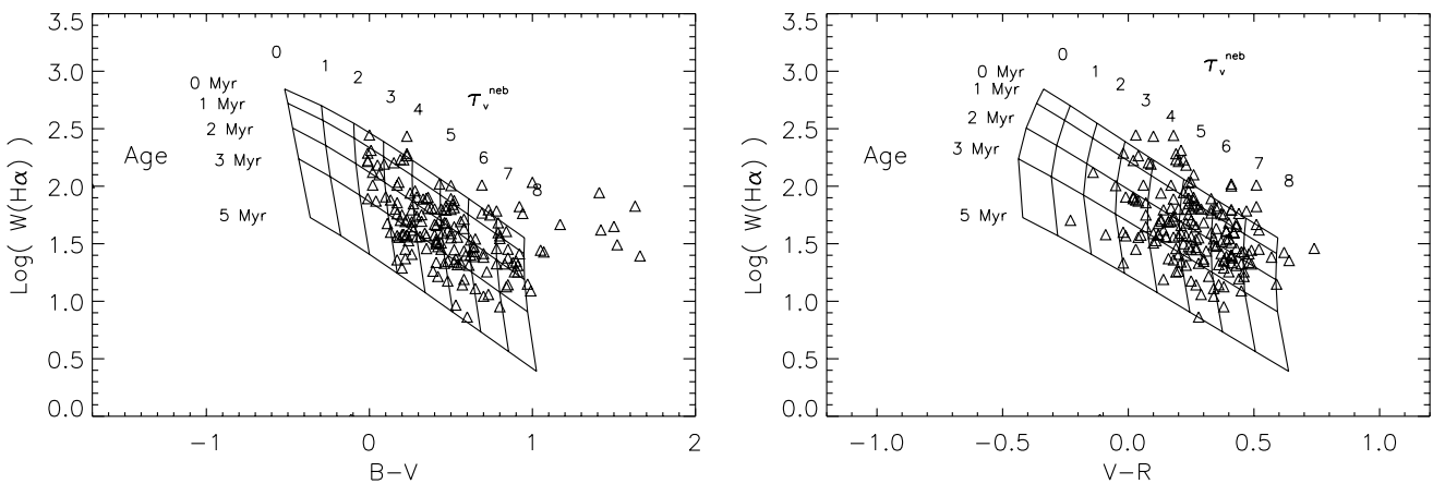
Fig. 8. Same as Fig. 7, but for \tau_V^{\text{stell}}/\tau_V^{\text{neb}} = 0.5 (see Sects. 3.3 and 5)
