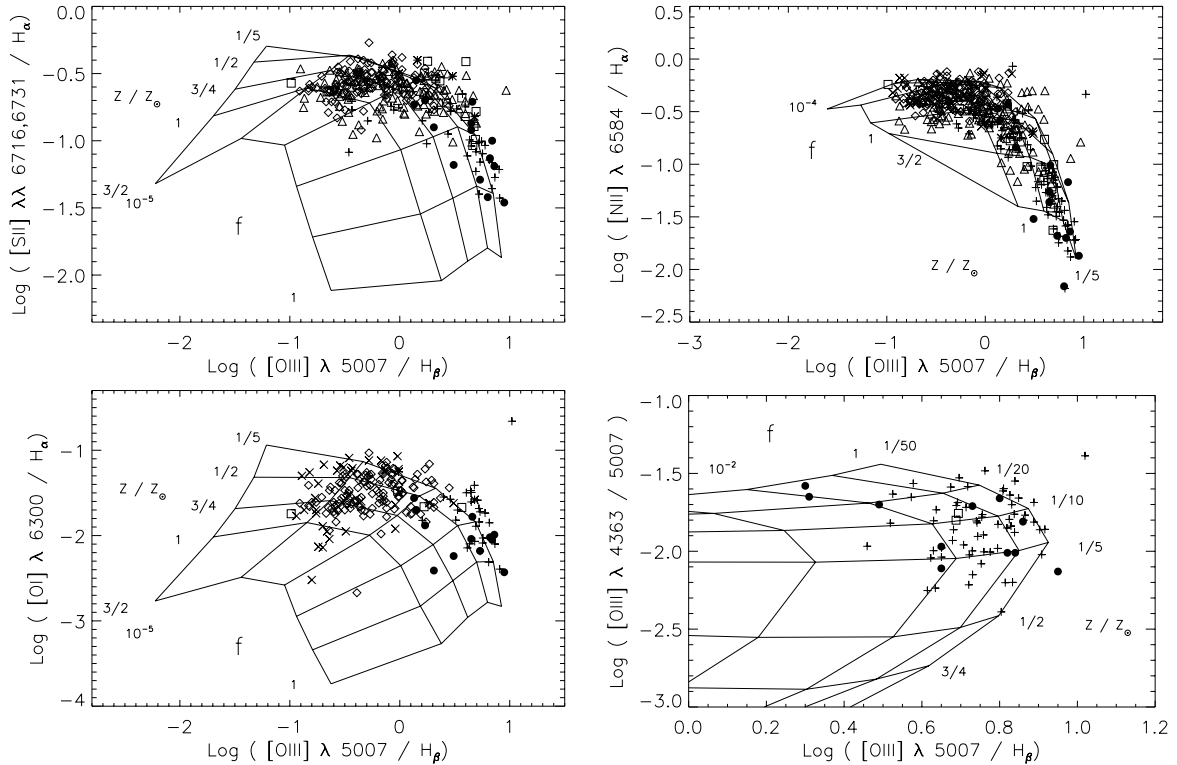
Fig. 1. Models of pure instantaneous starbursts for various filling factors ( f ) and metallicities ( Z ). The data are from Terlevich et al. (“plus” signs), Veilleux & Osterbrock (asterisks), French (filled circles), Veilleux et al. (diamonds), Contini et al. (triangles), Storchi-Bergmann et al. (squares) and Leech et al. (crosses)
