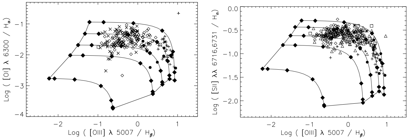
Fig. 3. Comparison of the data with five sequences obtained by varying the relative weights of the high ( f = 1 ) and low ( f = 10^{-5} ) excitation components. Solid diamonds are the points for which the low excitation component contributes to 0, 1, 10, 50, 90, 99 and 100% of the H\beta flux (from right to left)
