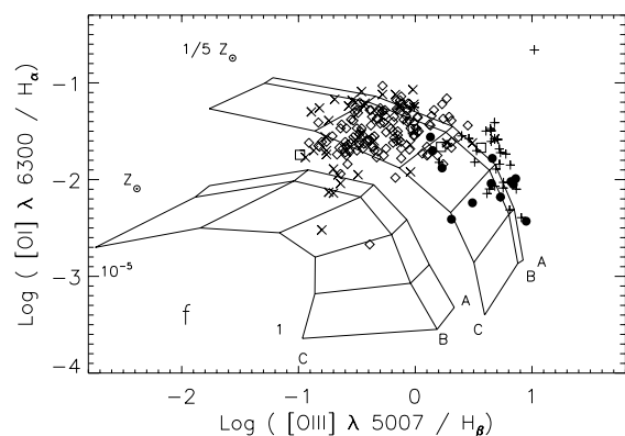
Fig. 6. Impact of the IMF on [O\ I]/H\alpha vs. [O\ III]/H\beta for two metallicities ( Z_{\odot}/5 and Z_{\odot} ). In each case, three f sequences are plotted: A ( \alpha = -2.35 , M_{low} = 0.1 M_{\odot} and M_{up} = 120 M_{\odot} ), B ( \alpha = -3.35 , M_{low} = 0.1 M_{\odot} and M_{up} = 120 M_{\odot} ) and C ( \alpha = -2.35 , M_{low} = 3 M_{\odot} and M_{up} = 30 M_{\odot} )
