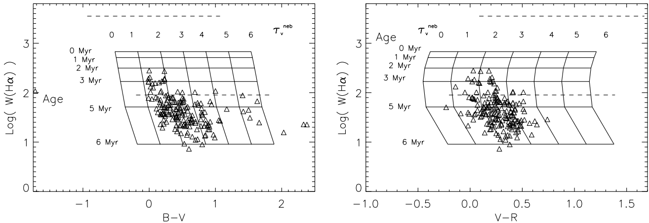
Fig. 7. Pure starburst models for various ages (0 to 6 Myr) and \tau_V between 0 to 6. The ratio \tau_V^{\text{stell}}/\tau_V^{\text{neb}} = 0.5 is equal to 1. The covering factor is 0.1. Data (triangles) are from Contini et al. (1998). The solid lines indicate the predictions of the \Omega/(4\pi) = 0.1 model grid. The two dashed lines show the t = 0 Myr (upper line) and t = 6 Myr (lower line) model results for \Omega/(4\pi) = 1
