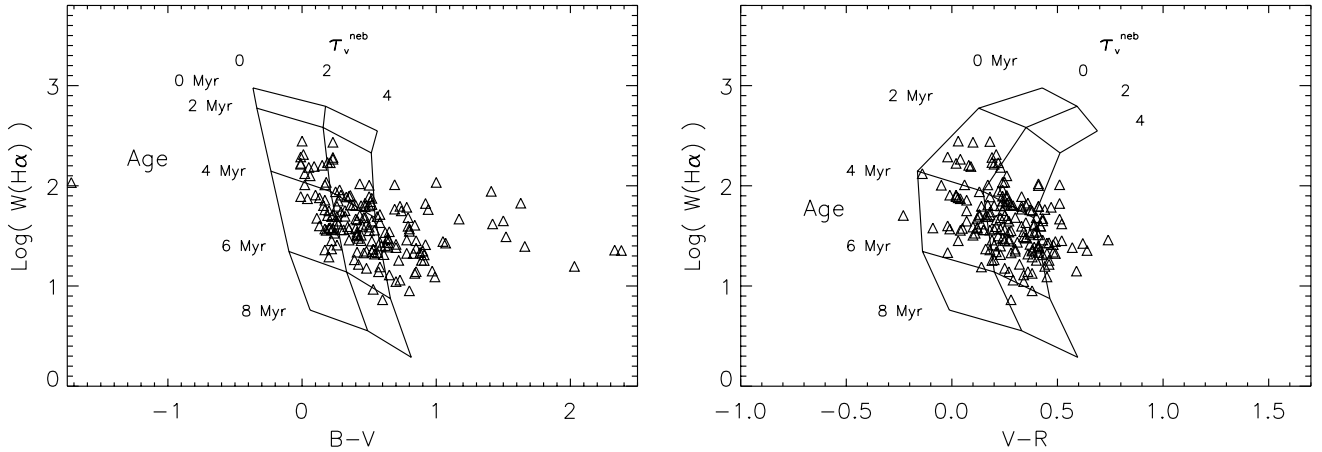
Fig. 9. H\alpha equivalent widths and colors for instantaneous + 100 Myr-old starbursts. The metallicity of the young starburst is solar. The old burst is assumed to have been ten times more intense than the current one. The model sequences are labeled in terms of the age of the present starburst and of the value of \tau_V^{neb}
