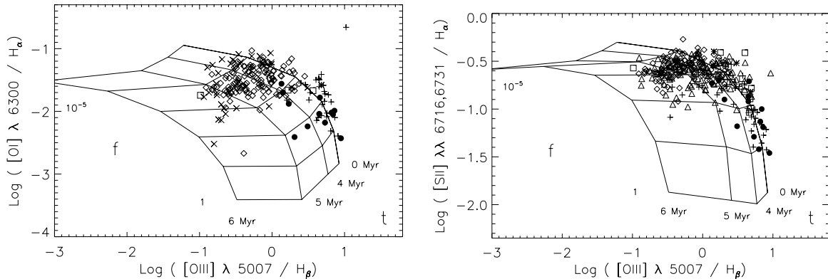
Fig. 4. Evolution with the starburst age of the Z_{\odot}/5 -model sequence plotted in Fig. 1
