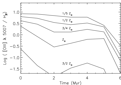
Fig. 5. Time evolution of the [O\ III]_{\lambda 5007}/H\beta ratio for instantaneous starbursts. The decrease of the ratio after 5 Myr is very rapid and puts severe constraints on the age of starbursts (see text for details)
