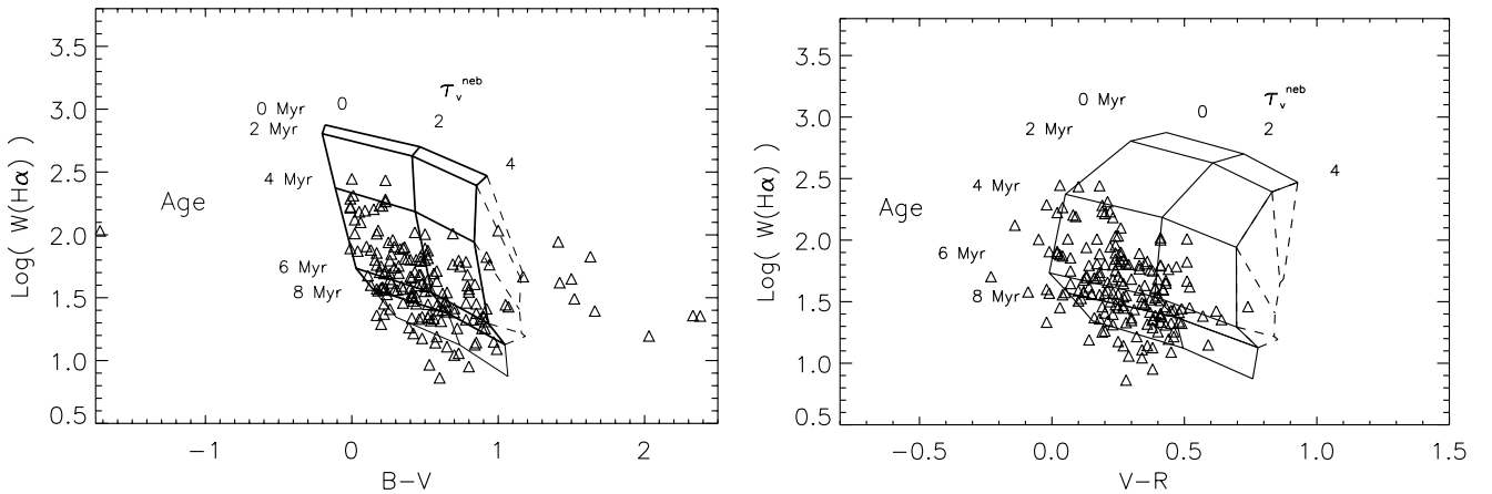
Fig. 10. H\alpha equivalent widths and colors for instantaneous burst + continuous star formation scenarios. The thick solid lines show the predictions of model D for different ages and extinction levels of the burst. The metallicity of the burst is 1/2 Z_{\odot} . The dashed lines indicate the shift of the right part of the grid when the contribution of the underlying population is increased (model C). The thin solid lines show the shift of the low part of the grid when the metallicity is equal to 3/2 Z_{\odot}
