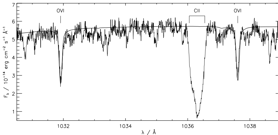
Fig. 3. O VI lines in the spectrum of Feige 55 displayed together with a model spectrum. The individual exposures were shifted according to the orbital motion and co-added. Therefore, the interstellar C II line is artificially broadened. There are also several other weak photospheric lines present.
