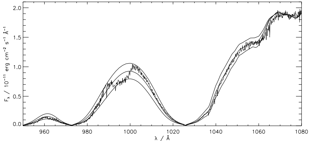
Fig. 4. FUSE spectra of CD -38^\circ 10980, rebinned to 0.15 \text{ \AA} resolution, and compared with three model atmospheres for DA white dwarfs of 23 000, 24 000, 25 000 K, \log g = 8.0 , normalized at 1070 \text{ \AA} .
