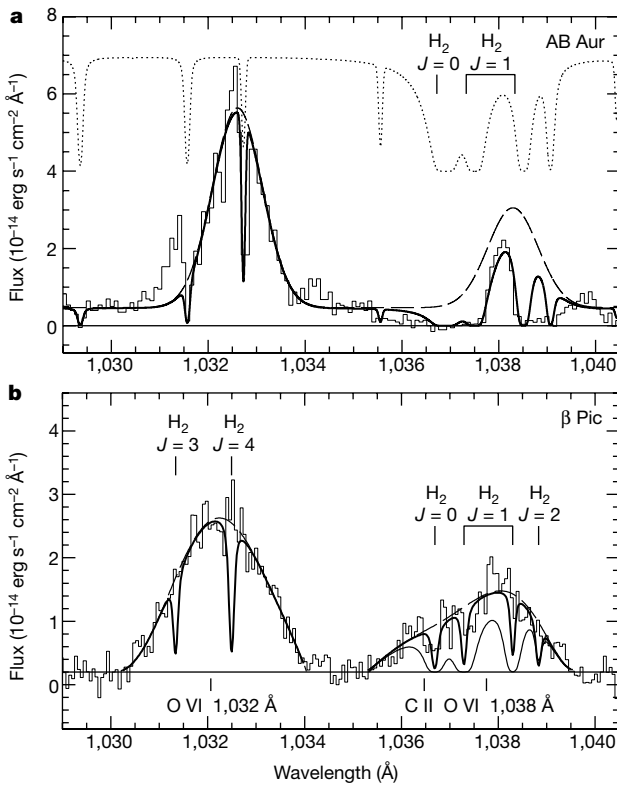
Figure 2 Plot of the observed \text{O VI} emission doublet and \text{H}_2 absorption lines. a , For the Herbig star AB Aur 20 , the \text{O VI} line at 1,032 Å is well fitted by a gaussian (dashed line). The \text{O VI} emission line at 1,038 Å is almost completely absorbed by a \text{H}_2 column density of N(\text{H}_2) = 7 \times 10^{19} \text{ cm}^{-2} . The normalized \text{H}_2 model is shown with a dotted line. Only a small window between the two J = 1 lines of \text{H}_2 allows a fraction of the emission to be seen (solid line). b , For \beta Pic, the wide \text{O VI} and \text{C II} emission lines are fitted with a polynomial (dashed line). The flux ratio of the two \text{O VI} lines is close to the theoretical value of 2, providing a direct indication of the low column density of \text{H}_2 . The thick solid line shows the expected spectrum for a \text{H}_2 column density of N(\text{H}_2) = 10^{18} \text{ cm}^{-2} in each J -level. Except for J = 0 , such a high column density is excluded at more than the 99% confidence level. The thin solid line shows the modelled spectrum if \text{H}_2 were present with a total column density of 5 \times 10^{19} \text{ cm}^{-2} and a temperature of 109 K, as given by the ISO observations of the 17- and 28- \mu\text{m} emission lines 1 . At this temperature, 34% of the \text{H}_2 molecules are at J = 0 , whereas 64% are at J = 1 . The total column density of 5 \times 10^{19} \text{ cm}^{-2} is actually only one-tenth of the lowest possible \text{H}_2 column density indicated by the ISO observations, if the \text{H}_2 were co-spatial with the dust. Such a model is rejected at more than \sim 20\sigma . If the \text{H}_2 detected by ISO were uniformly distributed in the disk, the \text{O VI} emission line at 1,038 Å would be completely absorbed and rendered undetectable in the present observation.
