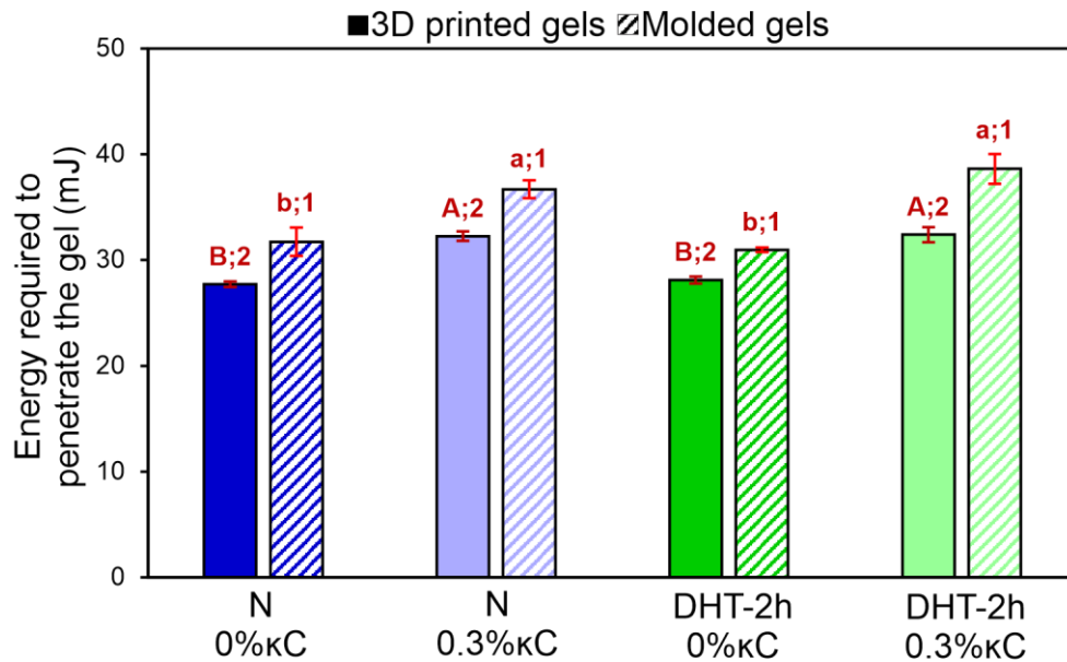
Figure 5: Energy required to penetrate the gel (mJ) obtained from the fork test using a texture analyzer attachment on 3D printed and molded cuboids for previously selected gels based on starch/ \kappa C/milk: native (N) + 0 or 0.3% \kappa C; and DHT-2h + 0 or 0.3% \kappa C. Gelling ingredients ( \kappa C + starch) was fixed in 5%. Statistical analysis by Tukey's test ( p < 0.05 ): different big caps indicate a significant difference between the 3D printed gels for the different treatments; different small caps indicate a significant difference between the molded gels for the different treatments; different numbers indicate significant difference between 3D printed and molded gels for the same treatment.
