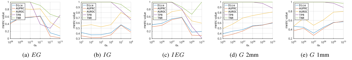
Fig. 2: Loss weight \alpha_A influence. Metrics (Dice, AUROC, AUPRC, TPR, TNR) versus \alpha_A for different attribution methods. Experiments was performed on validation 2mm (+1mm for gradient) tumors set.
