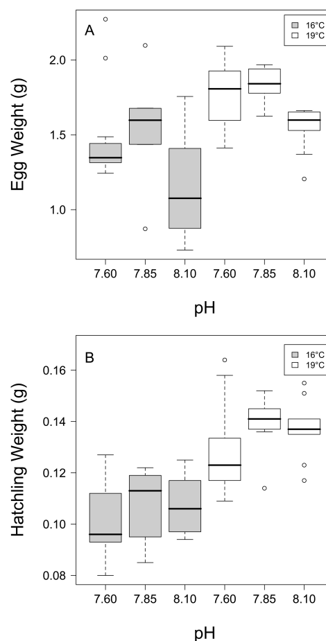
Fig. 1. Sepia officinalis . Weight (g) (A) of the eggs at the end of development ( n = 10 ) and (B) of the hatchlings ( n = 10 ) reared at different treatments different pH – pH 8.10, pH 7.85, pH 7.60 – for two temperatures, i.e. 16°C (grey) and 19°C (white). Results of the statistical analysis were reported on the Table 1.
