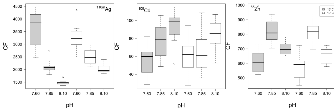
Fig. 2. Sepia officinalis . Concentration factors of ^{110\text{m}}\text{Ag} , ^{109}\text{Cd} and ^{65}\text{Zn} (CF; n = 10 ), in the newly hatched juvenile exposed at three different pH – pH 8.10, pH 7.85, pH 7.60 – for two temperatures, i.e. 16°C (grey) and 19°C (white). Results of the statistical analysis were reported on the Table 1.
