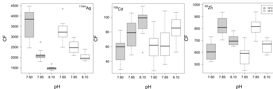
Fig. 2. Sepia officinalis . Concentration factors of ^{110m}\text{Ag} , ^{109}\text{Cd} and ^{65}\text{Zn} (CF; n = 10 ), in the newly hatched juvenile exposed at three different pH – pH 8.10, pH 7.85, pH 7.60 – for two temperatures, i.e. 16°C (grey) and 19°C (white). Results of the statistical analysis were reported on the Table 1.
