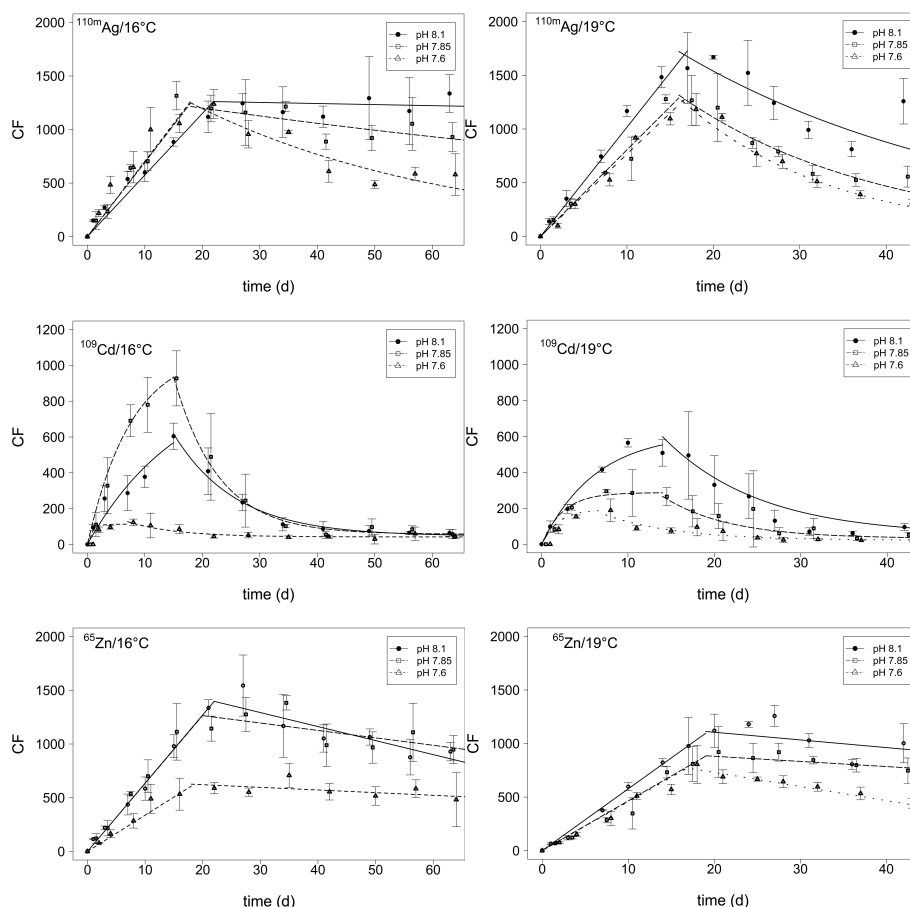
Fig. 3. Sepia officinalis . ^{110m}\text{Ag} , ^{109}\text{Cd} and ^{65}\text{Zn} uptake kinetics (CF; mean \pm SD; n = 3 ) in the eggshell from eggs exposed at three different pH – pH 8.10 (●), pH 7.85 (□), pH 7.60 (▲) – for two temperatures, i.e. 16°C (left side) and 19°C (right side).
