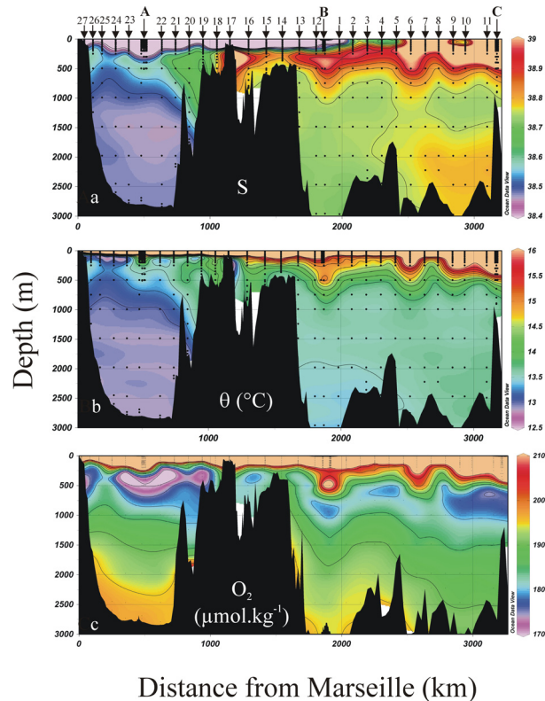
Fig. 2. Property distributions along the 2008 BOUM transect going from Marseille (France; Station 27; distance is 0 km) to the Levantine Basin (south of Cyprus Island; Station C; distance from Marseille is ~3200 km). (a) Salinity ( S ); (b) potential temperature ( \theta ; °C); and (c) concentration of dissolved oxygen ( O_2 ; \mu\text{mol.kg}^{-1} ). Stations along the transect are indicated above panel (a) .
