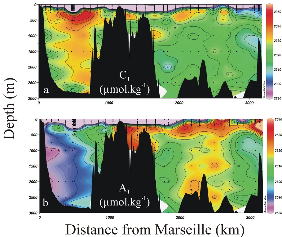
Fig. 5. (a) Distribution of the total dissolved inorganic carbon ( C_T , \mu\text{mol kg}^{-1} ); (b) distribution of the total alkalinity ( A_T ; \mu\text{mol kg}^{-1} ).
