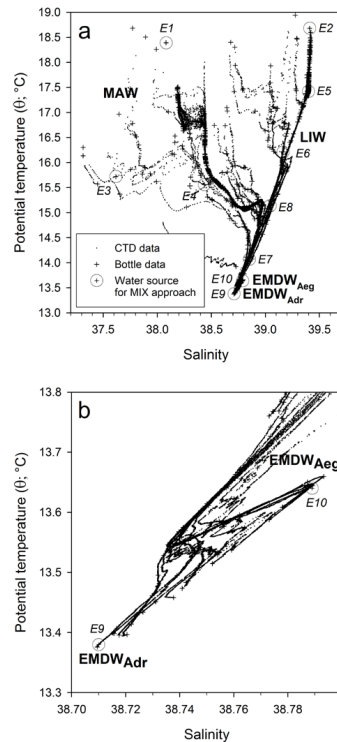
Fig. 4. Diagram \theta/S for the Eastern Mediterranean Sea where CTD and bottle data are all represented. The main water masses (MAW, LIW, EMDW Adr , and EMDW Aeg ) described in the text and the 10 water sources (from E1 to E10) used by the MIX approach are also indicated. Panel (b) is a zoom of (a) in order to better visualize EMDW Adr and EMDW Aeg .
