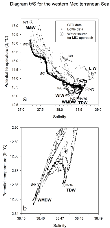
Fig. 3. Diagram \theta/S for the Western Mediterranean Sea where CTD and bottle data are all represented. The main water masses (MAW, WIW, LIW, TDW, and WMDW) described in the text and the 10 water sources (from W1 to W10) used by the MIX approach are also indicated. Panel (b) is a zoom of (a) in order to better visualize WMDW and TDW.
