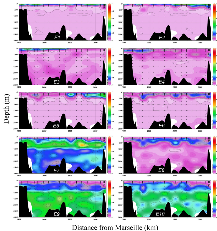
Fig. 9. Results of the MIX approach. Distribution of the mixing coefficient ( k_j ) of each water source (from E1 to E10) in the Eastern Mediterranean Sea.
