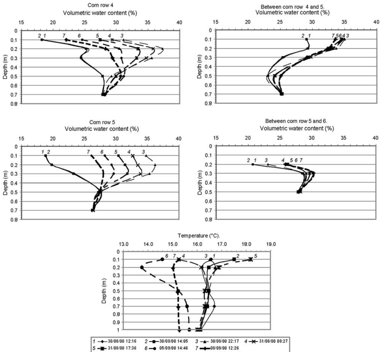
Figure 9. Volumetric moisture and thermal profile changes over time.
